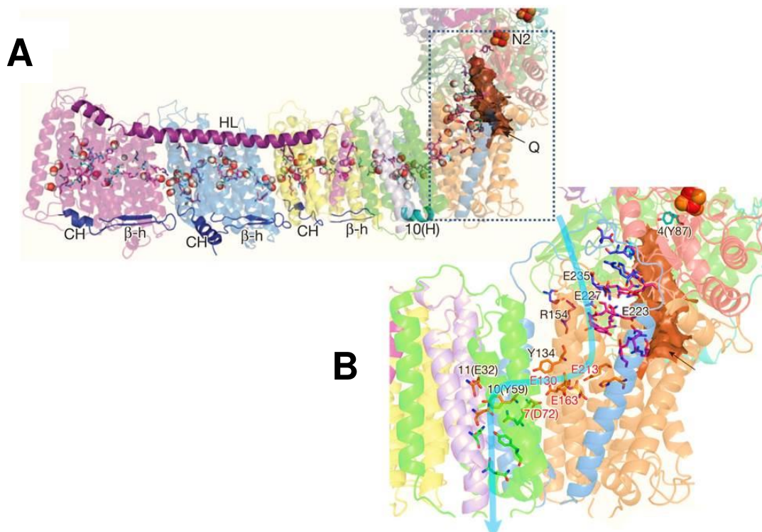
Figure 1.15: E-channel and central hydrophilic axis of Complex I. Cartoon representation of the atomic model (Protein Data Bank identifier 4HEA) at 3.3 Å resolution from T. thermophilus . A ) Central axis of charged and polar residues (charged residues have carbon in magenta, polar in cyan). Residues shown are either central to half-channels or are forming the connection between them. Predicted waters nearby are shown as spheres. Connecting elements are shown in solid colors: helix HL in magenta and the \beta H element in blue, with the C-terminal helix CH and the \beta -harping ( \beta -h) from each antiporter labelled. B ) Charged and polar residues constituting the channel are shown as sticks. Quinone cavity is shown with surface in brown and approximate proton translocation path is indicated by blue arrow. Key residues are labelled, with the Glu/Asp quartet in red. Residues are numbered according to the Thermus thermophilus structure [Nqo8 subunit of T.thermophilus (ND1 subunit in B. taurus ): Glu130 (Ser110), Tyr134 (Tyr114), Arg154 (Arg134), Glu213 (Glu192), Glu223 (Glu202), Glu227 (Glu216), Glu235 (Glu224)]; [Nqo7 subunit of T. thermophilus (ND3 subunit in B. taurus ): Asp72 (Asp66)]; [Nqo10 subunit of T. thermophilus (ND6 subunit in B. taurus ): Tyr59 (Tyr60)]. [from Baradaran et al, 2013]
