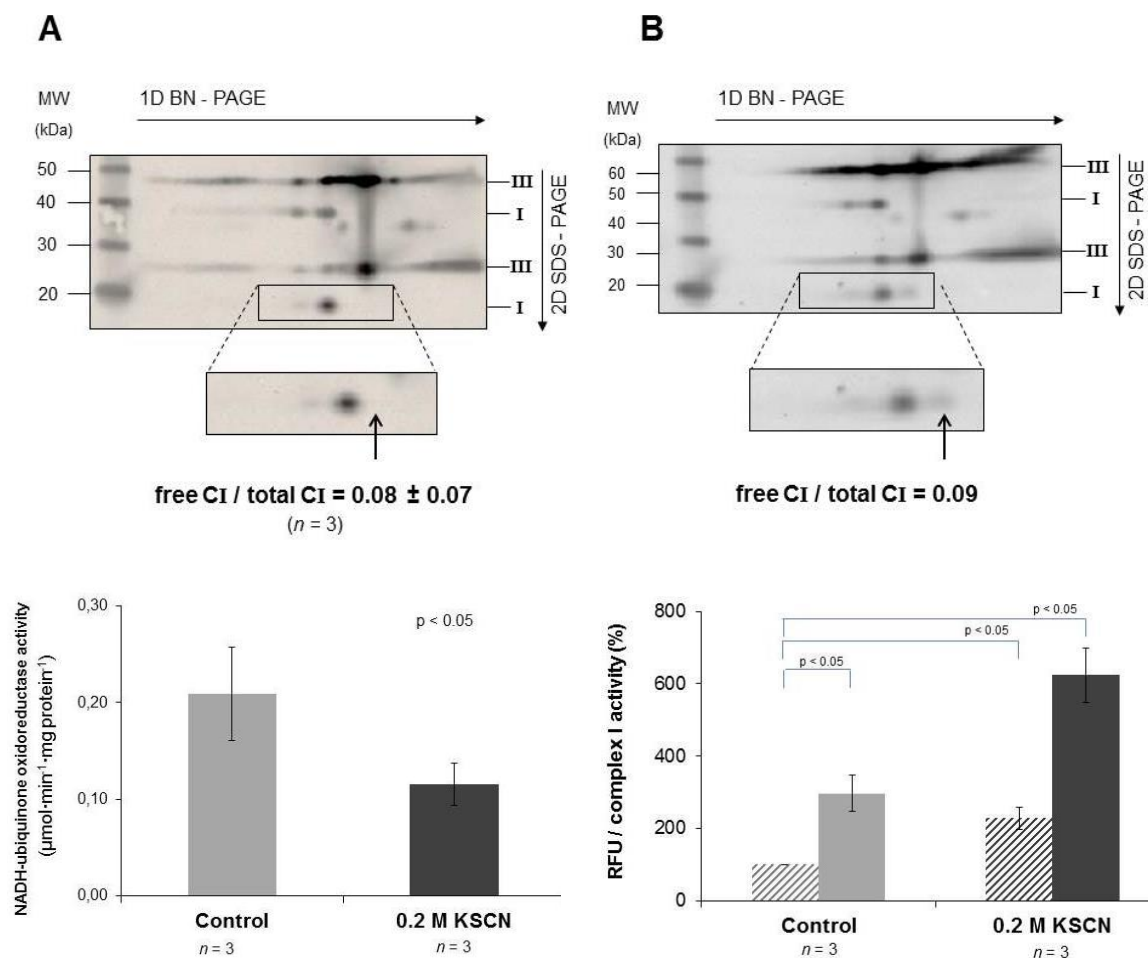
Figure 3.12: Disassembling of supercomplex I I III 2 in R4B 1:1 proteoliposomes after treatment with 0.2 M KSCN. (A) Respiratory supercomplexes and complexes from KSCN-treated R4B 1:1 were solubilized with digitonin with a detergent to protein ratio (w:w) of 8 and resolved by western blotting after 2D BN/SDS-PAGE followed by immunodetection using monoclonal antibodies specific for single respiratory subunits. The image shown in the picture was obtained in camera by double overlaying exposures (not postproduction computer-graphic overlay) to the antibody against the NDUFA9 (39 kDa) and NDUFB8 (20 kDa) subunits of Complex I and, in sequence, to the antibodies against the Rieske protein (22 kDa) and Core protein 2 (47 kDa) of Complex III. Arrows point to monomeric Complex I. The ratio of free Complex I versus total Complex I (free CI / total CI) were determined by densitometric analysis of the immunoblots as described in the section “Materials and Methods”. (B) Potassium thiocyanate dependence of NADH-ubiquinone oxidoreductase activity, measured after removal of KSCN by ultracentrifugation. Activity rates are expressed in \mu\text{moles of NADH}\cdot\text{min}^{-1}\cdot\text{mg protein}^{-1} (D) The production of hydrogen peroxide was measured, after removal of KSCN by ultracentrifugation, in the presence of 1.8 \mu\text{M} mucidin (dashed bars) and 1.8 \mu\text{M} mucidin plus 4 \mu\text{M} rotenone (solid bars). Values are expressed as relative fluorescence intensity (RFU) by DCF normalized against Complex I activity and shown as percentage values of the reference sample ( i.e. control R4B 1:1 in the presence of mucidin only). Data are given as mean \pm S.D. n shows the number of independent samples. p -values were calculated using the Student’s t -test.
