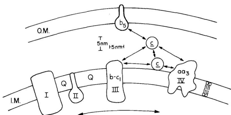
Figure 1.5: Random collision model of Hackenbrock (1986). Structural arrangement of mitochondrial respiratory components [Hackenbrock et al, 1986]. O.M: outer membrane, I.M.: inner membrane, b 5 : cytochrome b 5 , c : cytochrome c , Q: ubiquinone, I, II, III, IV: complexes I, II, III, and IV, respectively
