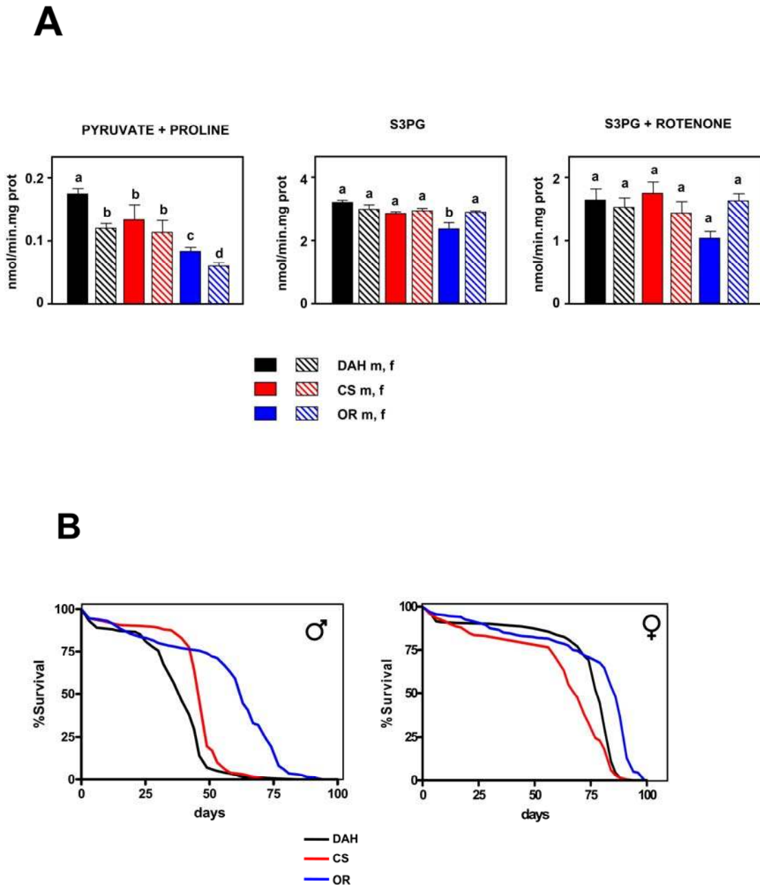
Figure 1. Mitochondrial ROS production versus lifespan in three wild type strains of Drosophila melanogaster . (A) Rate of mtROS production (assayed as H_2O_2 , mean \pm SEM). a, b, c and d indicate statistically significant differences between groups (ANOVA, p < 0.05 , n = 5-9 samples per group), m: male, f: female. (B) Survival curves. Combined data from two independent experiments using 100 flies per group per experiment. Mean, maximum lifespans (d) were: DAH males (39, 49); CS males (46, 53); OR males (63, 74); DAH females (79, 84); CS females (69, 81); OR females (86, 91).
