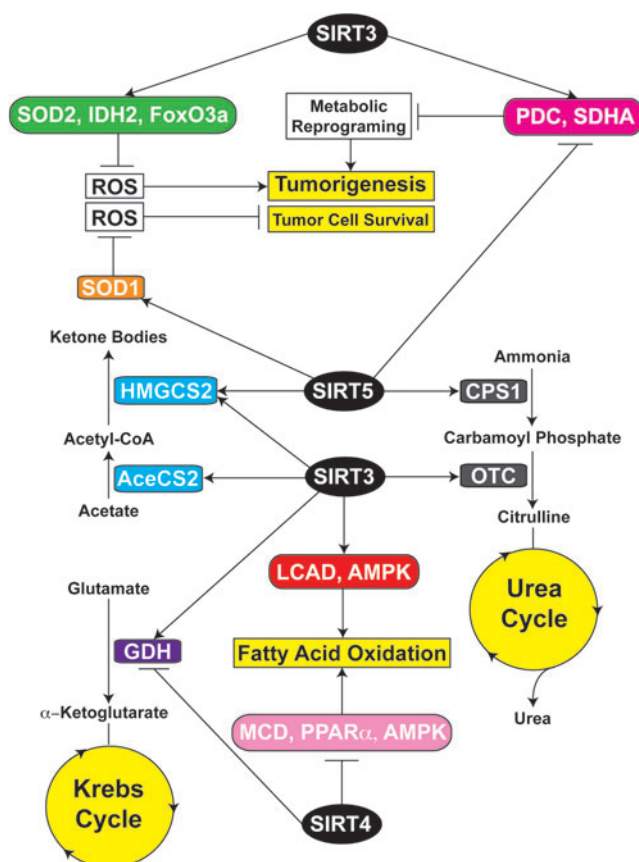
FIG. 6. Overview of interplay between mitochondrial sirtuins. Enzymes involved in ketogenesis (blue boxes) and urea cycle (gray boxes) are activated by both SIRT3 and SIRT5. While SIRT5 inhibits the enzymatic activities of glucose metabolism (magenta box), SIRT3 activates them to suppress metabolic reprogramming and tumorigenesis. SIRT3 also suppresses tumorigenesis by decreasing ROS levels through activation of antioxidant machinery (green box). SIRT5 activates SOD1 (orange box) to maintain ROS below toxic levels to support tumor cell survival. SIRT3 also shares common target/pathways with SIRT4. SIRT3 promotes FAO by activating LCAD and AMPK (red box), whereas SIRT4 represses FAO through inhibition of MCD, PPAR \alpha , and AMPK (pink box). Similarly, SIRT3 activates GDH (violet box), which is inhibited by SIRT4. To see this illustration in color, the reader is referred to the web version of this article at www.liebertpub.com/ars
