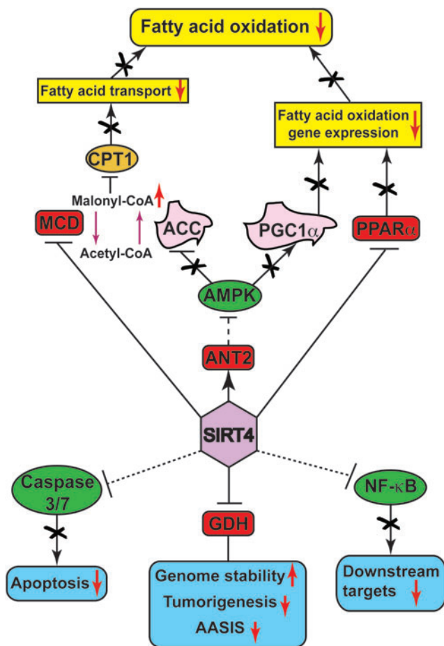
FIG. 4. Overview of SIRT4 target substrates and cellular functions. SIRT4 directly (red rounded rectangles) or indirectly (green ellipses) modulates the activity of various target substrates, which either regulate aspects of fatty acid metabolism (yellow rectangles) or play crucial roles in other cellular processes (blue rounded rectangles). Upward and downward red arrows indicate the promotion or suppression of a particular activity, gene expression, or physiological activity. To see this illustration in color, the reader is referred to the web version of this article at www.liebertpub.com/ars
