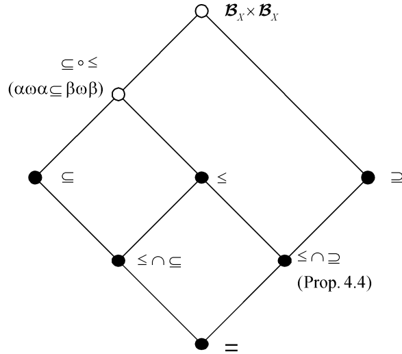
Fig. 1. A sublattice of preorders on \mathcal{B}_X . Filled circles denote orders.
