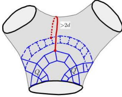
FIGURE 1. Double injectivity radius > d at \mathcal{Q} = \{Q, Q'\} .
