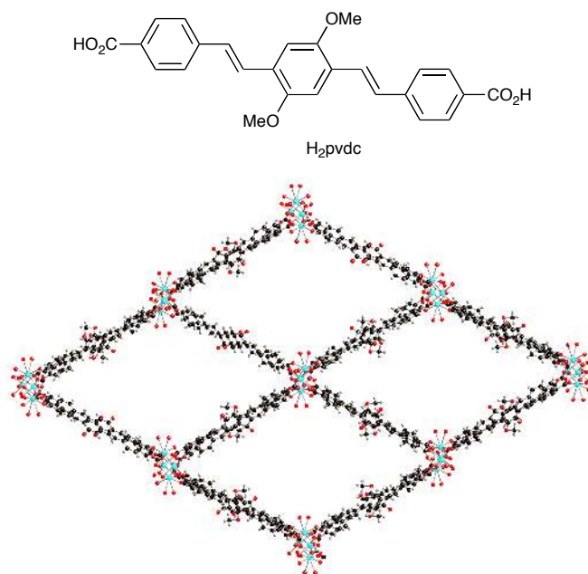
Figure 18. Part of the structure of [\text{Yb}_2(\text{pvdc})_3(\text{H}_2\text{O})_2] 93 , with ytterbium atoms cyan, oxygen atoms red, carbon atoms black and hydrogen atoms grey.
