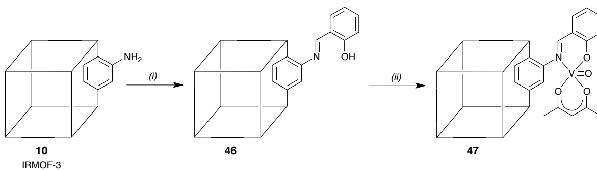
Scheme 4. (i) salicylaldehyde, toluene; (ii) VO(acac) 2 , CH 2 Cl 2 .
