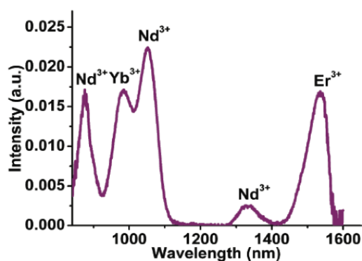
Figure 19. \text{Yb}^{3+} , \text{Er}^{3+} and \text{Nd}^{3+} emission from [\text{Nd}_{0.18}\text{Er}_{1.10}\text{Yb}_{0.72}(\text{pvdc})_3(\text{H}_2\text{O})_2] 94 ( \lambda_{\text{ex}} = 490 \text{ nm} ). Reprinted with permission from ref. 74 .
