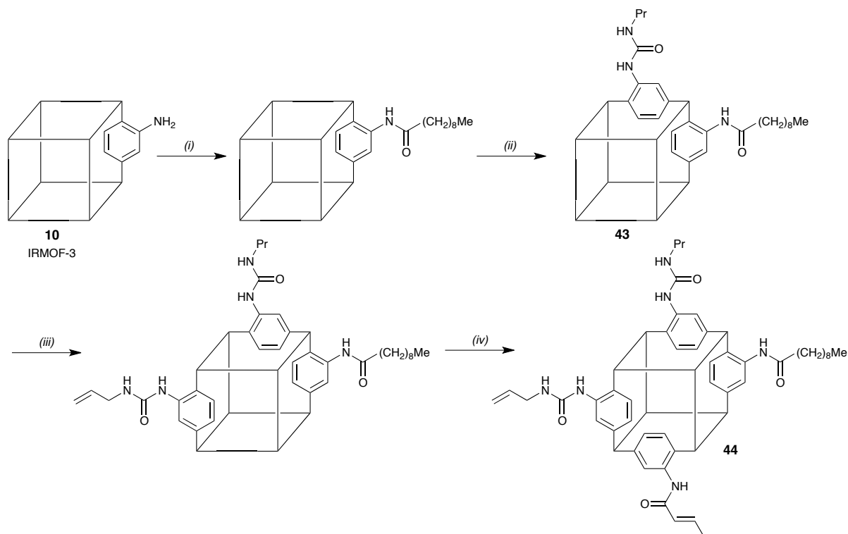
Scheme 2. (i) \text{O}\{\text{C(O)(CH}_2\text{)}_8\text{Me}\}_2 , \text{CHCl}_3 ; (ii) \text{PrNCO} , \text{CHCl}_3 ; (iii) \text{CH}_2=\text{CHCH}_2\text{NCO} , \text{CHCl}_3 ; (iv) \text{O}\{\text{C(O)CH}=\text{CHMe}\}_2 , \text{CHCl}_3 .
