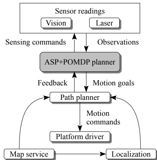
Fig. 10: Pictorial representation of a subset of nodes in the ROS implementation of our architecture.
