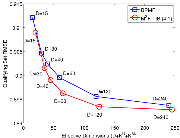
Figure 3. RMSE performance of BPMF and M 3 F-TIB with (K^U, K^M) = (4, 1) on the Netflix Prize Qualifying set as a function of the number of parameters modeled per user or item.
