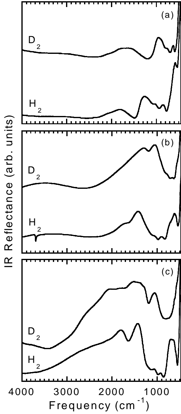
Figure 3. Internal reflectance infrared spectra of (a) 400 nm Mn-Mg, (b) 385 nm Fe-Mg, (c) 250 nm Co-Mg films on ZnSe substrates following loading in H 2 and D 2 .
