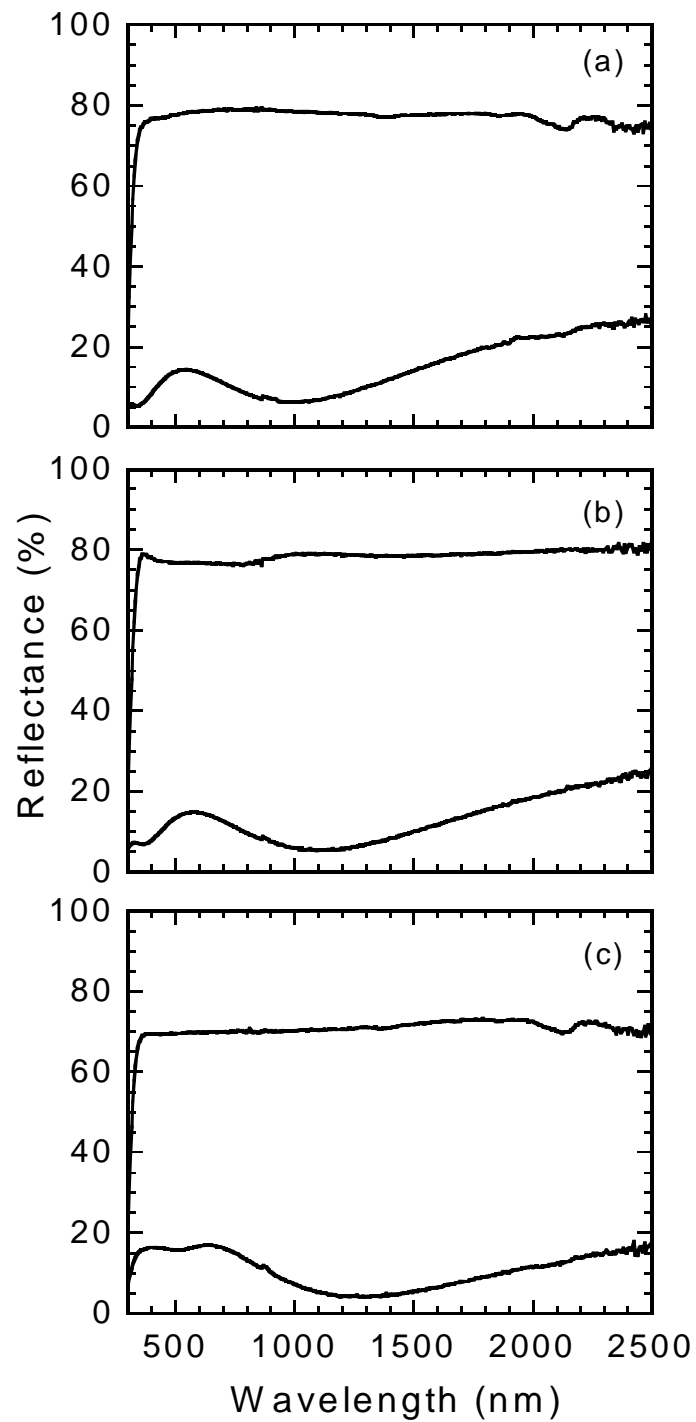
Figure 1. Vis-NIR reflectance spectra of (a) 60 nm Mn-Mg, (b) 40 nm Fe-Mg, (c) 40 nm Co-Mg films (T:Mg ca. 1:6) with 7 nm Pd overlayers on glass substrates in the metallic (upper curve) and hydride (lower curve) states. Spectra were recorded from the substrate side.
