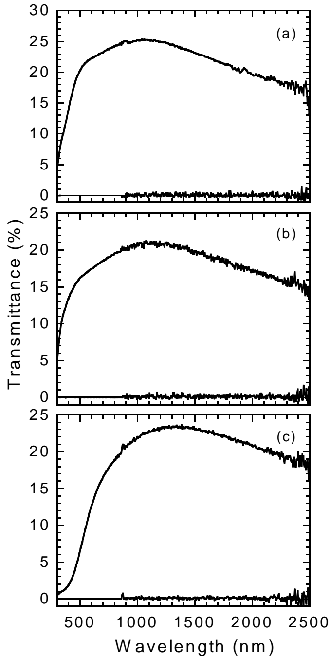
Figure 2. Vis-NIR transmittance spectra of (a) 60 nm Mn-Mg, (b) 40 nm Fe-Mg, (c) 40 nm Co-Mg films (T:Mg ca. 1:6) with 7 nm Pd overlayers on glass substrates in metallic (lower curve) and hydride (upper curve) states.
