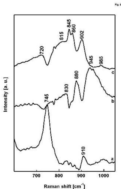
Figure 9 Spectral components according to the SIMPLISMA analysis of the set of 500 Raman spectra: a.) \text{MoO}_2 -like oxide, b.) amorphous \text{Mo}_5\text{O}_{14} -type oxide, and c.) \text{Mo}_5\text{O}_{14} -type oxide.
