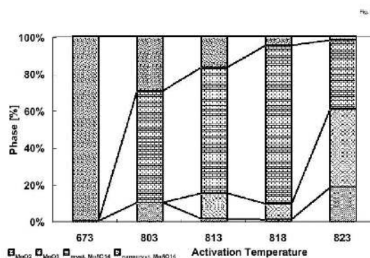
Figure 2 Quantitative XRD phase analysis of the crystalline parts of the mixed oxide catalysts activated at different temperatures
