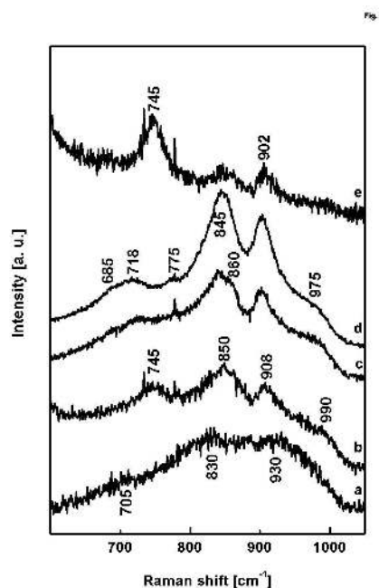
Figure 8 Raman spectra of the starting material and the samples thermally activated at the temperatures indicated: a.) starting material, b.) activated at 803 K, c.) activated at 813 K, d.) activated at 823 K, and e.) activated at 829 K.
