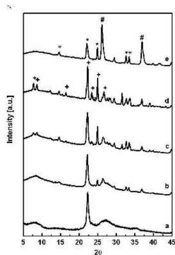
Figure 1 XRD pattern of the starting material and catalysts activated at temperatures indicated: a.) starting material, b) 803 K, c.) 813 K, d.) 818 K, e.) 823 K. The reflections of \text{Mo}_5\text{O}_{14} (+), \text{MoO}_2 (#) and \text{MoO}_3 (*) are indicated.
