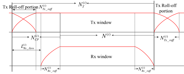
Fig. 1. The illustration of transmit and receive windows.
