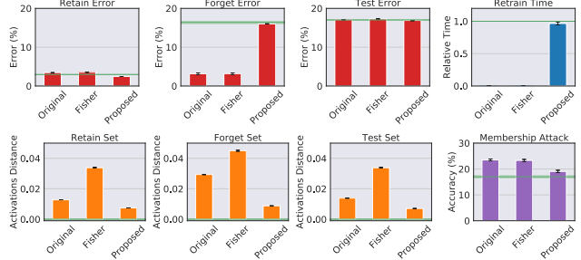
Figure 3. Read-out functions for different forgetting methods. We forget a subset of 10% of the training data through 10 equally-size sequential deletion requests using different forgetting methods, and show the value of the several readout functions for the resulting scrubbed models. Ideally, the value of the readout function should be the same as the value (denoted with the green area) obtained on a model retrained from scratch without those samples. Closer to the green area is better. (Original) denotes the trivial baseline where we do not apply any forgetting procedure. (Fisher) Adds Fisher noise as described in ([15]). (ML-Forgetting) The model obtained with our method after forgetting. In all cases, we observe that ML-Forgetting obtains a model that is indistinguishable from one trained from scratch without the data, whereas the other methods fail to do so. This is particularly the case for the Retrain Time readout functions, which exploits full knowledge of the weights and it is therefore more difficult to defend against.
