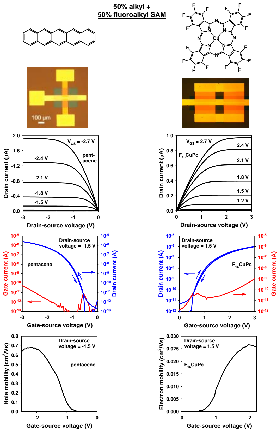
Figure S5. Transistor characteristics. Photographs and electrical characteristics of a pentacene p-channel TFT with a channel length of 30\ \mu\text{m} and a channel width of 100\ \mu\text{m} (left) and of a F_{16}CuPc n-channel TFT with a channel length of 30\ \mu\text{m} and a channel width of 1000\ \mu\text{m} (right). For the optimum SAM gate dielectric composition (50% alkyl phosphonic acid + 50% fluoroalkyl phosphonic acid), the threshold voltages of the TFTs are symmetric with respect to V_{GS} = 0\ \text{V} .
