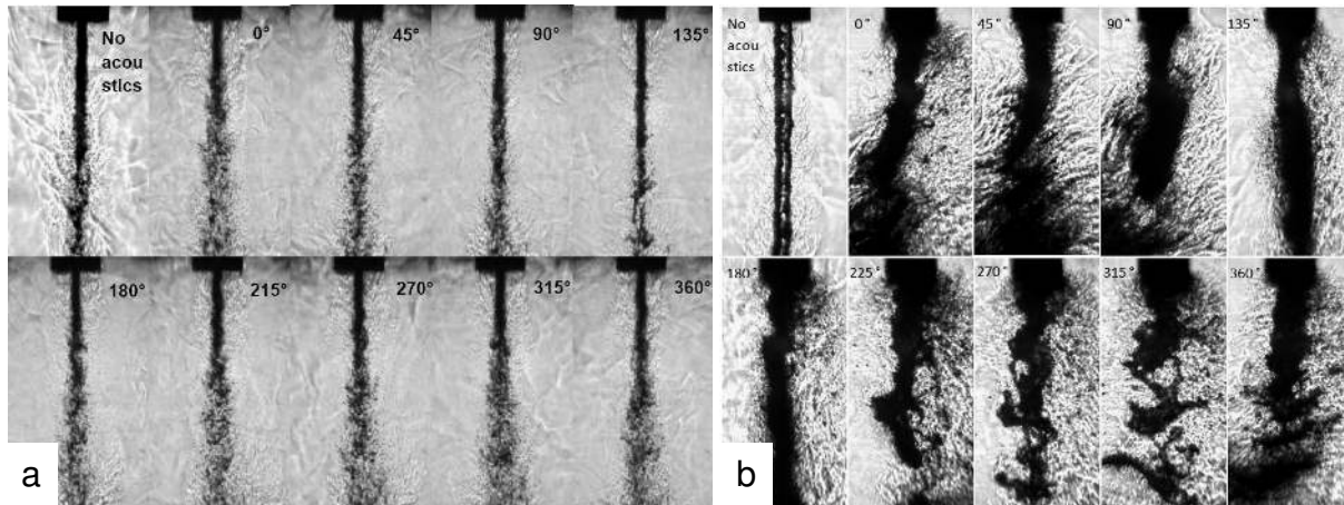
Figure 6.a. Collection of subcritical coaxial jet images at P_{\text{chamber}} = 1.50 \text{ MPa} , J = 0.17 with original injector geometry. b. Images with P_{\text{chamber}} = 1.48 \text{ MPa} , J = 0.089 with new injector geometry.
