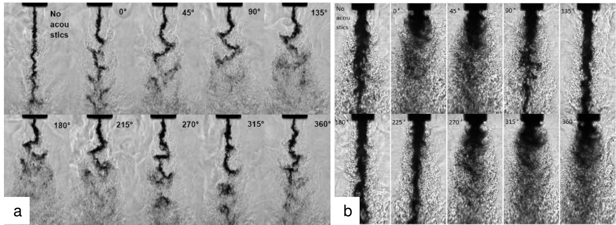
Figure 7.a. Collection of subcritical coaxial jet images at P_{\text{chamber}} = 1.45 \text{ MPa} , J = 2.6 with original injector geometry. b. Images at P_{\text{chamber}} = 1.49 \text{ MPa} , J = 2.0 with new injector geometry.
