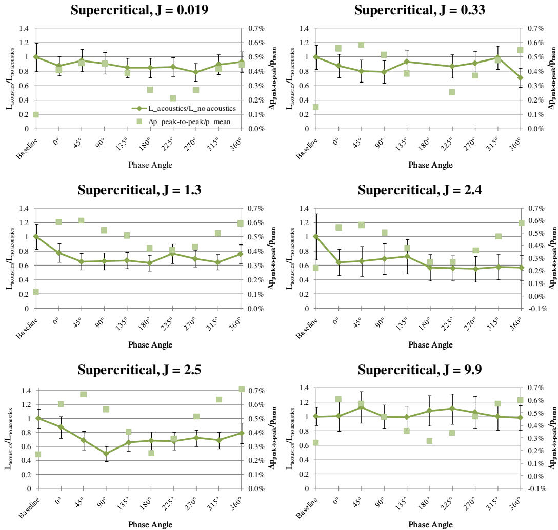
Figure 15. Dark core length with acoustics ( L_{acoustics} ) over dark core length without acoustics ( L_{no\ acoustics} ), shown in diamonds, versus phase angle between acoustic sources for supercritical pressures. The the peak-to-peak pressure perturbation as a percentage of the mean chamber pressure ( \Delta p_{peak-to-peak}/p_{mean} ), in squares, is also plotted. Original injector geometry.
