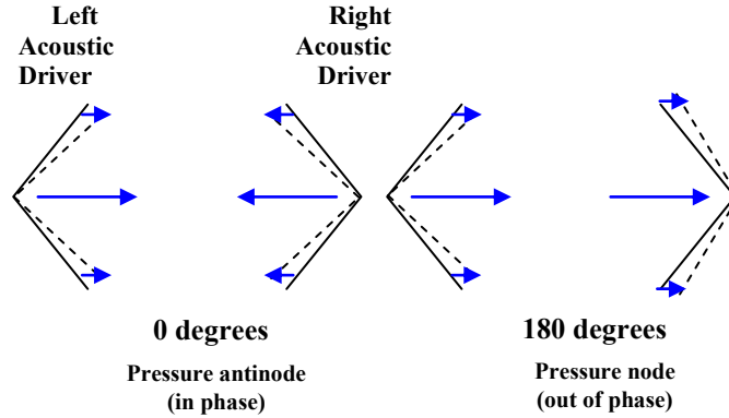
Figure 5. Simplified diagram of the two acoustic drivers at a 0^\circ and 180^\circ phase angle, indicating relative flow perturbation directions.
