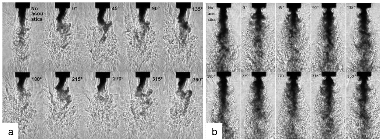
Figure 8.a. Collection of subcritical coaxial jet images at P_{\text{chamber}} = 1.50 \text{ MPa} , J = 9.6 with original injector geometry. b. Images at P_{\text{chamber}} = 1.49 \text{ MPa} , J = 7.8 with the new injector geometry.
