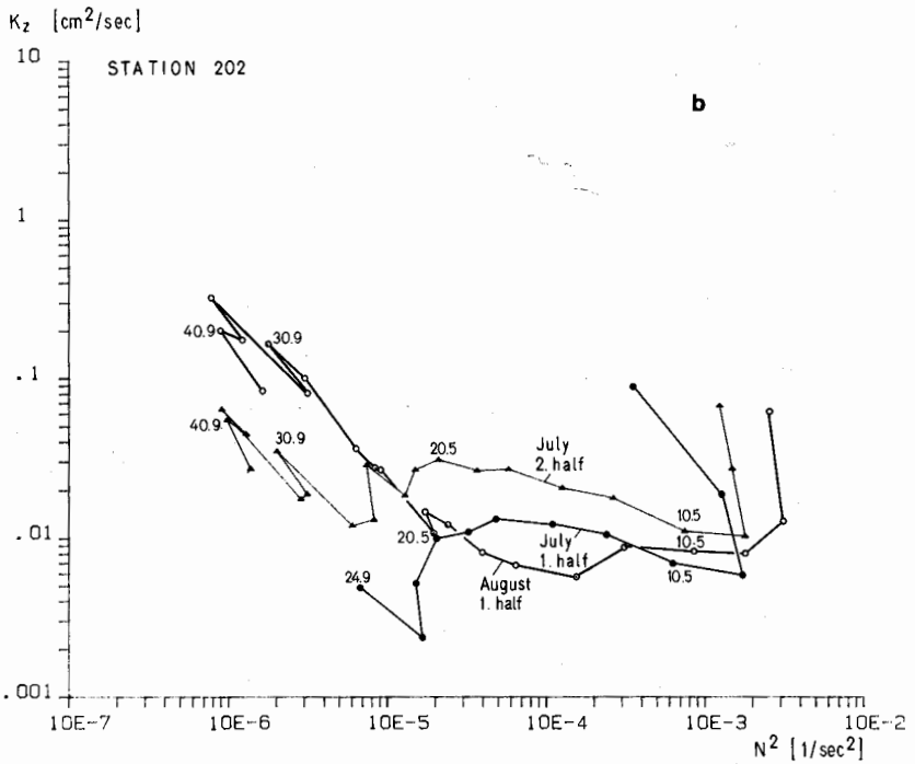
Figure 12. Vertical eddy-diffusion coefficients K_z versus the square of the Brunt-Väisälä frequency N^2 . Numbers indicate water depth (meters).
