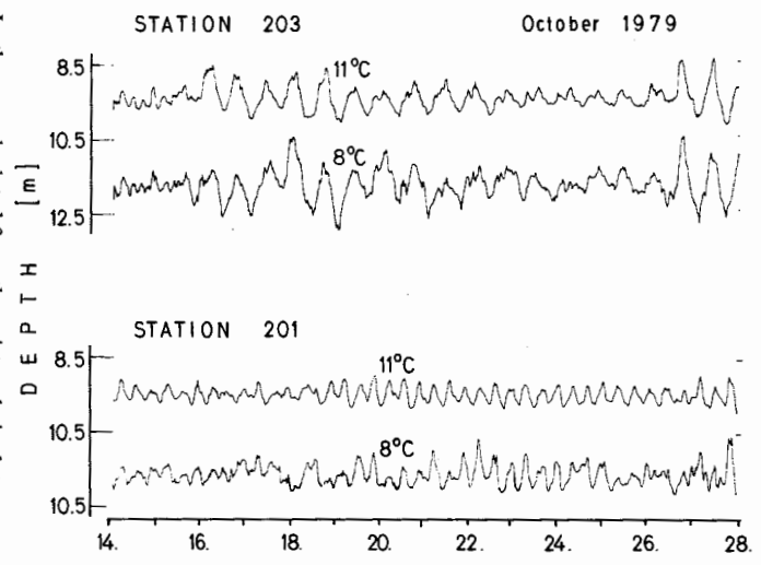
Figure 13. Isotherms calculated from thermistor chain data.
