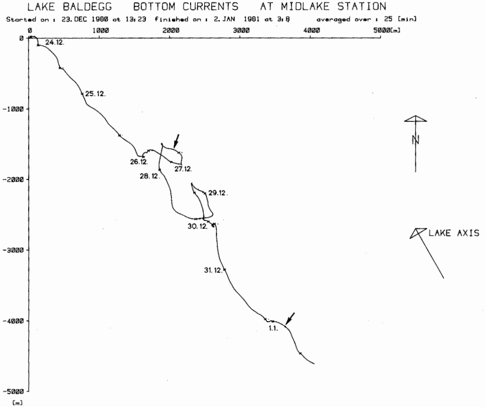
Figure 19. Progressive vector diagram of the bottom currents for the period 23 December 1980 to 2 January 1981; 12-h time intervals are marked on the curve. Dates given at every second mark refer to the time of 13.31 hours. Current speeds have been averaged over five consecutive measurements. Arrows indicate onset of 'particle rain' (see text).
