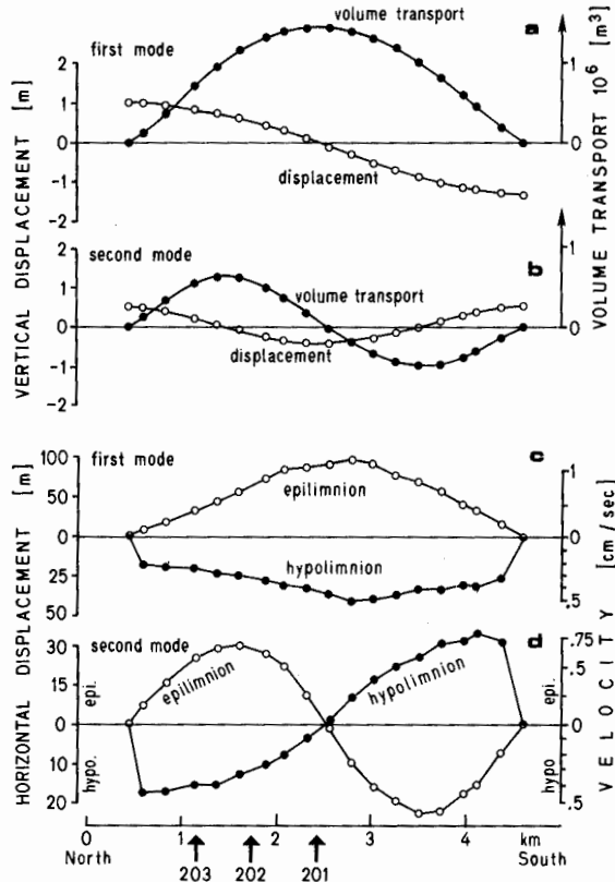
Figure 15. Defant model calculation for the first (uninodal) and the second (binodal) internal seiche mode in a two-layer model of Lake Baldegg. Interface depth: 15 m; epilimnion temperature: 12 °C; hypolimnion temperature: 5 °C. Arrows on the bottom indicate the position of thermistor chain stations along the lake axis.
