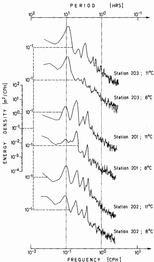
Figure 14. Isotherm energy spectra for the period from 14 October to 28 October 1979. Station number and isotherm temperature are marked on each curve.
