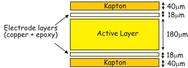
Figure 9: Sequence of layers for the MFC. Approximate data provided by Smart Material
