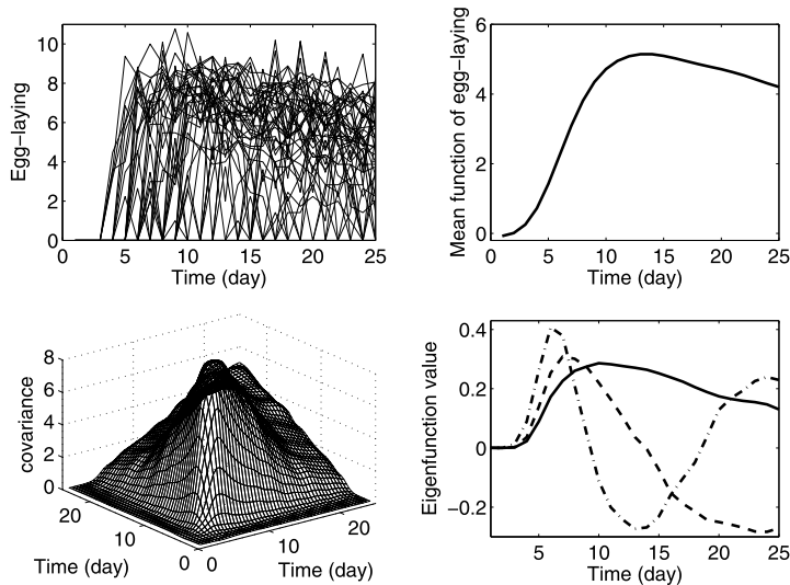
FIG. 1. Top-left: Daily egg-laying counts, after square-root transformation, for 50 randomly selected flies for the first 25 days of their lifespan. Top-right: Smooth estimate of the mean function. Bottom-left: Smooth nonnegative definite estimate of the covariance surface. Bottom-right: Smooth estimates of the first (solid), second (dashed) and third (dash-dotted) eigenfunctions, explaining 95% of the total variation.
