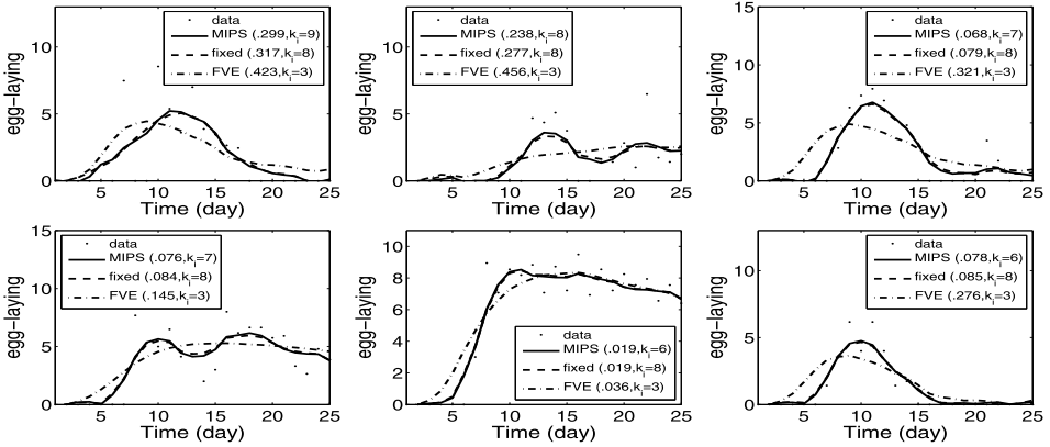
FIG. 2. Daily egg-laying counts for six randomly selected flies for the first 25 days of their lifespan, overlaid with the smooth estimates obtained from the proposed functional mixture model (MIPS), solid line, from functional principal component analysis with a fixed number of 8 components, dashed line, and for a fixed number of three components which explain 95% of the total variation, dash-dotted line. Shown in parentheses are the individual relative squared errors and the included number of components for that individual.
