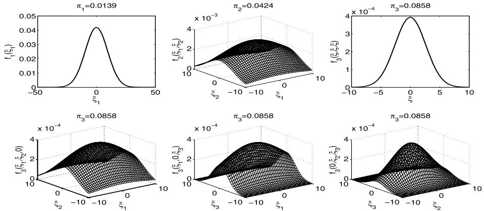
FIG. 3. Estimated probability density function for the first three mixture components and their corresponding mixture proportions \pi_k . Top: left, the probability density function of the first component; middle, the probability density function of the second component; right, the diagonal of the probability density function of the third component. Bottom: 2-dimension slices of the probability densities of the third component at \xi_1 = 0 , \xi_2 = 0 and \xi_3 = 0 , respectively, in the left, middle and right panels.
