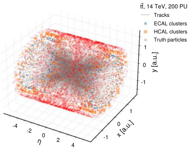
Fig. 1 A simulated t\bar{t} event from the MLPF dataset with 200 PU interactions. The input tracks are shown in gray, with the trajectory curvature being defined by the inner and outer \eta, \phi coordinates. Electromagnetic (hadron) calorimeter clusters are shown in blue (orange), with the size corresponding to cluster energy for visualization purposes. We also show the locations of the generator particles (all types) with red cross markers. The radii and thus the x, y -coordinates of the tracker, ECAL and HCAL surfaces are arbitrary for visualization purposes
