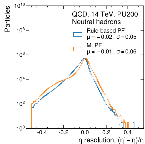
Fig. 10 The energy and \eta resolution of the DELPHESPF benchmark and the MLPF model for neutral hadrons in simulated QCD multijet events with PU. Both reconstruction algorithms show comparable performance
