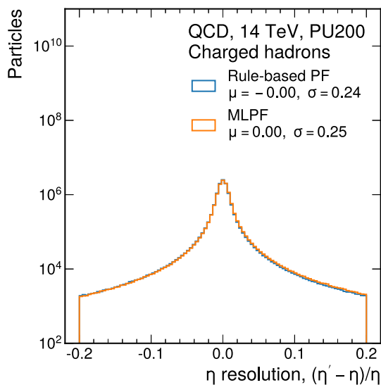
Fig. 9 The p_T and \eta resolution of the DELPHESPF benchmark and the MLPF model for charged hadrons in simulated QCD multijet events with PU. The p_T resolution is comparable for both algorithms, with the angular resolution being driven by the smearing of the track ( \eta, \phi ) coordinates
