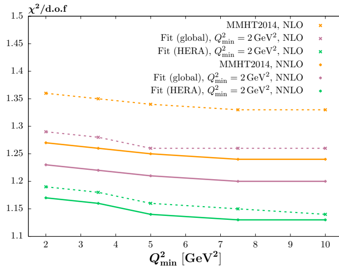
Figure 1: A comparison of \chi^2 per point for the three variations of NLO and NNLO fits, all with fixed lower Q_{\min}^2 = 2 \text{ GeV}^2 , for different Q_{\min}^2 on the HERA data used in the calculations.
