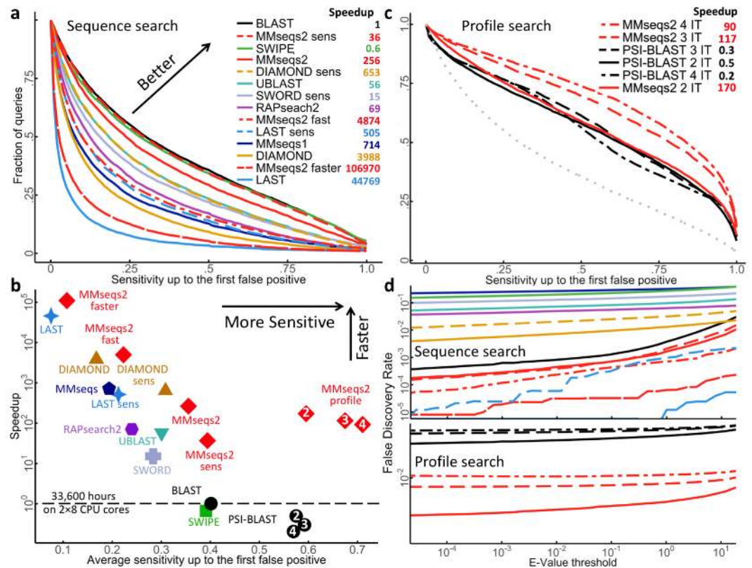
Figure 2: MMseqs2 pushes the boundaries of sensitivity-speed trade-off. a Cumulative distribution of Area under the curve (AUC) sensitivity for all 6370 searches with UniProt sequences through the database of 30.4 M full-length sequences. Higher curves signify higher sensitivity. Legend: speed-up factors relative to BLAST, measured on a 2×8 core 128 GB RAM server using a 100 times duplicated query set (637 000 sequences). Times to index the database have not been included. MMseqs2 indexing takes 11 minutes for 30.3M sequences of avg. length 342. b Average AUC sensitivity versus speed-up factor relative to BLAST. White numbers in plot symbols: number of search iterations. c Same analysis as in a , for iterative profile searches. d False discovery rates for sequence and profile searches. Colors: as in a (top) and c (bottom).
