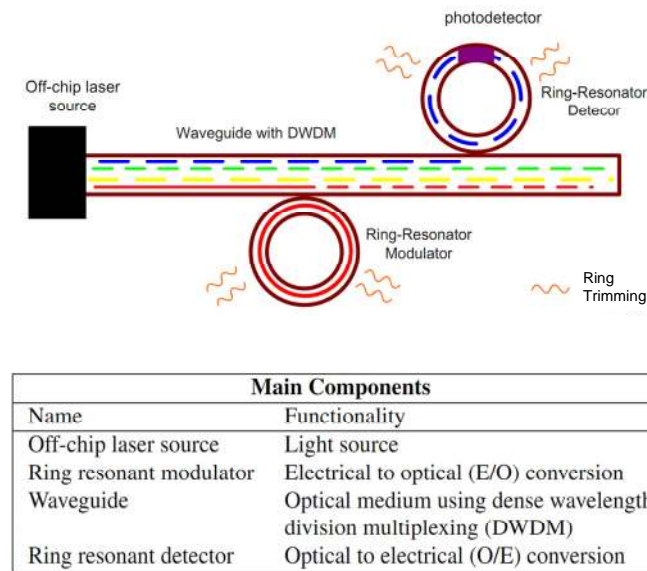
Fig. 1. Main Optical Components of Ring Resonator Nanophotonic Network-on-chip
