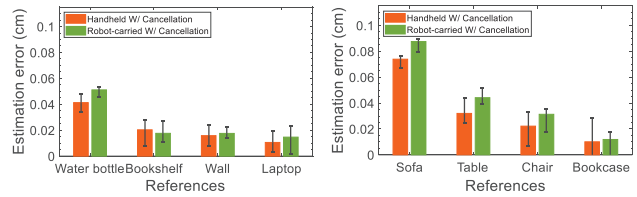
Figure 19: A lot of commonly seen objects in our environment can be selected as reference for device motion removal.
