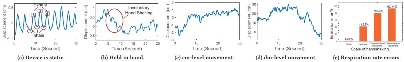
Figure 7: Respiration monitoring under different device movement conditions. Clear signal variation pattern corresponding to respiration cycles can be obtained when device is static and device movement corrupts the signal variation pattern.
