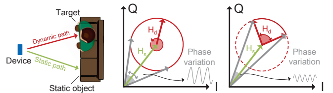
Figure 6: Dynamic signal vector ( H_d ) rotates with respect to the static signal vector ( H_s ).
