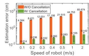
Figure 16: Effect of robot moving speed.
