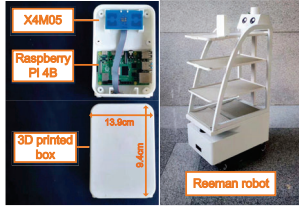
Figure 13: Hardware implementation.
