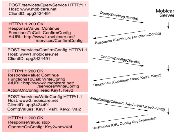
Figure 6: Configuration Service Protocol Exchange.
