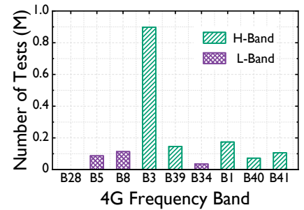
Figure 6: Number of access bandwidth tests conducted on each LTE band.
