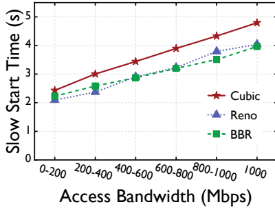
Figure 17: TCP slow start time for different congestion control algorithms.
