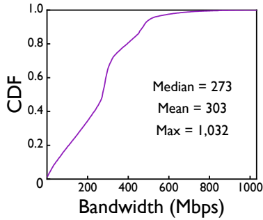
Figure 7: Bandwidth distribution for 5G access in our measurement.
