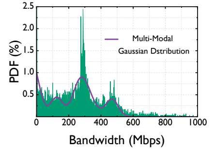
Figure 19: Probability distribution for 5G access bandwidths.
