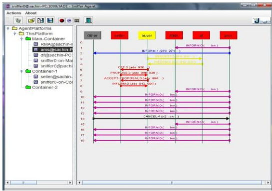
Fig 8.2 Message passing between the agents using the sniffer agent
