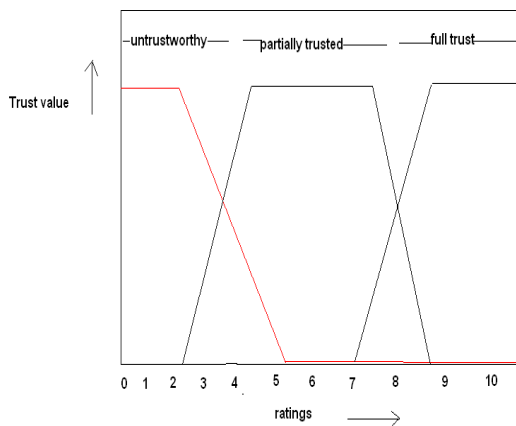
Fig 8.3 graph between ratings and Trust values
