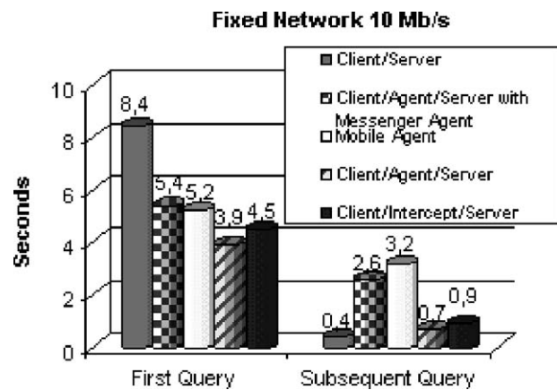
Chart 6. Mean times for 10 Mb/s client connectivity.
