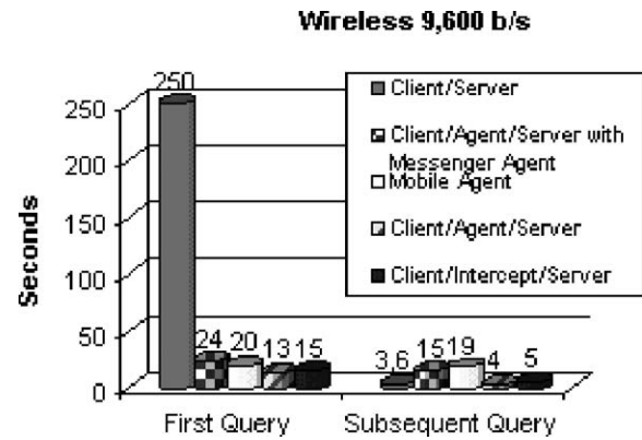
Chart 5. Mean times for 9,600 b/s client connectivity.
