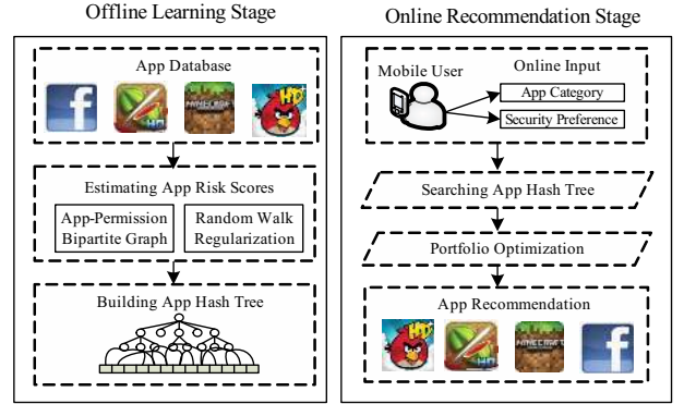
Figure 3: The recommendation framework.
