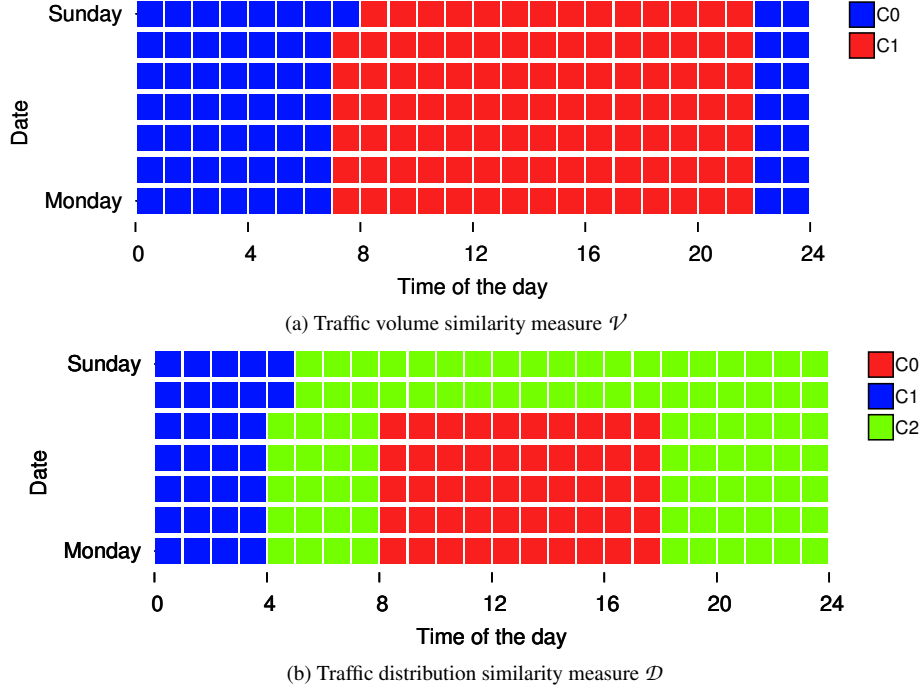
FIGURE 5: Mobile traffic profile categories defined on the training set \bar{\mathbb{T}}' . Each square represents one snapshot, and colors map to categories.
