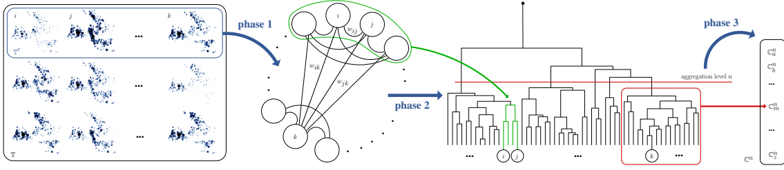
FIGURE 1: Workflow of the framework for the definition of categories of network usage profiles. Phase 1 : construction of the snapshot graph from snapshots (portrayed here as geographical plots of the mobile traffic volume) in the training set T' . Phase 2 : iterative aggregation of graph vertices into a dendrogram structure. Phase 3 : identification of the clustering level n granting the maximum separation between the groups of snapshots. The resulting clusters C_m^n \in C^n are mapped to network usage profile categories.
