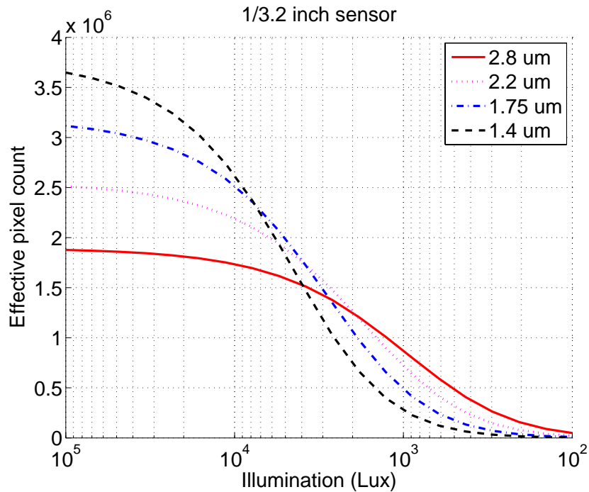
Fig. 1. Effective pixel count as a function of illumination level for imaging systems with 1/3.2 inch sensors at four different pixel sizes (2.8 \mu\text{m} , 2.2 \mu\text{m} , 1.75 \mu\text{m} and 1.4 \mu\text{m} ).
