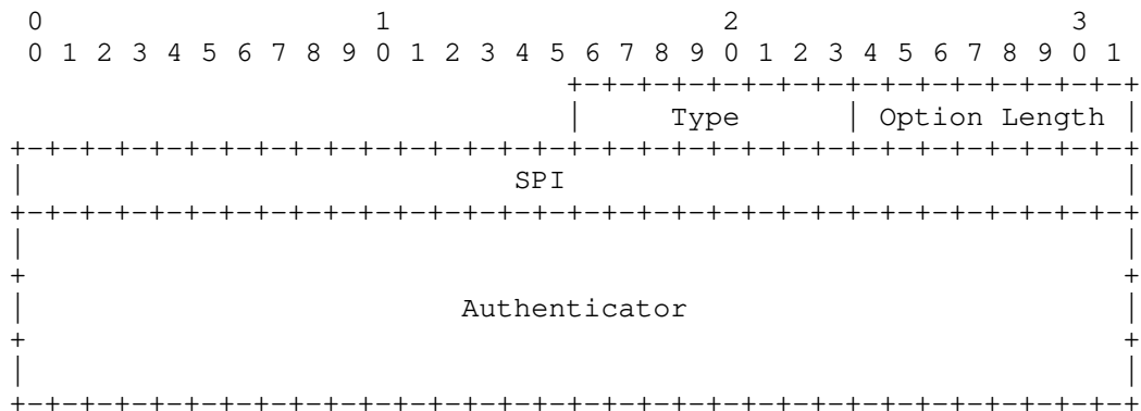
Figure 15: Binding Authorization Data for FMIPv6 (BADF) Option
