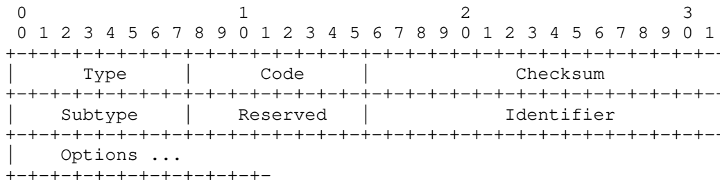
Figure 4: Router Solicitation for Proxy Advertisement (RtSolPr) Message
