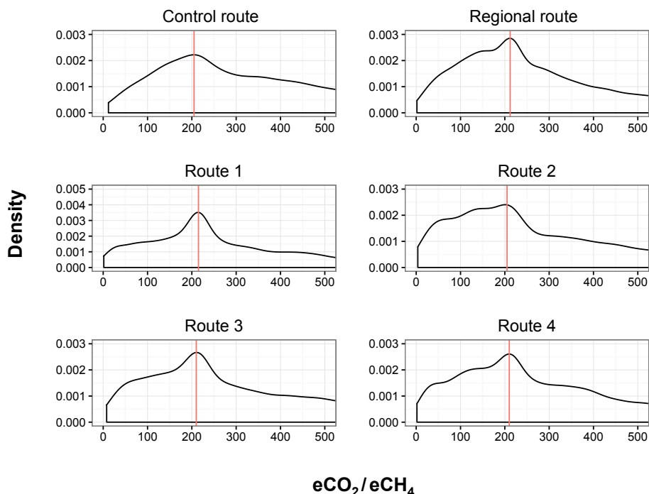
Figure 4. Kernel density plots showing the density of e\text{CO}_2 : e\text{CH}_4 measurements on each route. Red vertical lines indicate natural e\text{CO}_2 : e\text{CH}_4 values near 215. Methane-enriched peaks are visible to the left of the natural ratio on all routes except for the control, where the slope approaches zero with no peaks because we surveyed substantially less natural gas infrastructure on this route. Ratios higher than natural represent \text{CO}_2 -rich plumes which would be caused not by natural-gas-related emissions but likely by diluted car exhaust fumes or other industry types.
