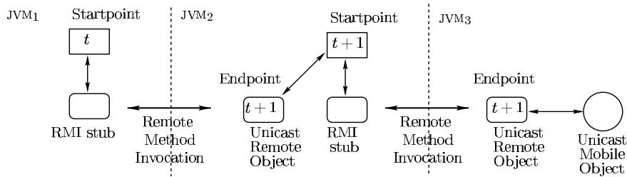
Fig. 3. Mobile object migration.
