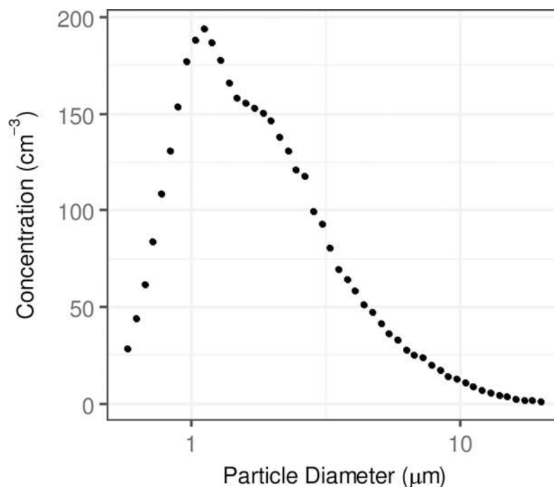
Fig 2. Total particle number size distribution of concrete dust particles as measured by the APS. The respective number size distributions were aggregated to the total size distribution.
