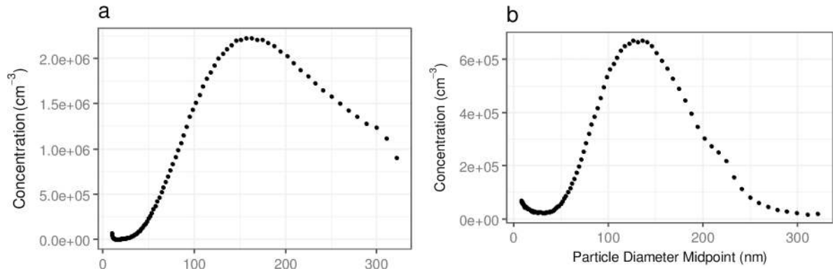
Fig 1. Particle size distributions as measured by the SMPS for a) Cigarette smoke particles b) Petrol exhaust particles. The respective number size distributions for different times were aggregated to the total size distribution.
