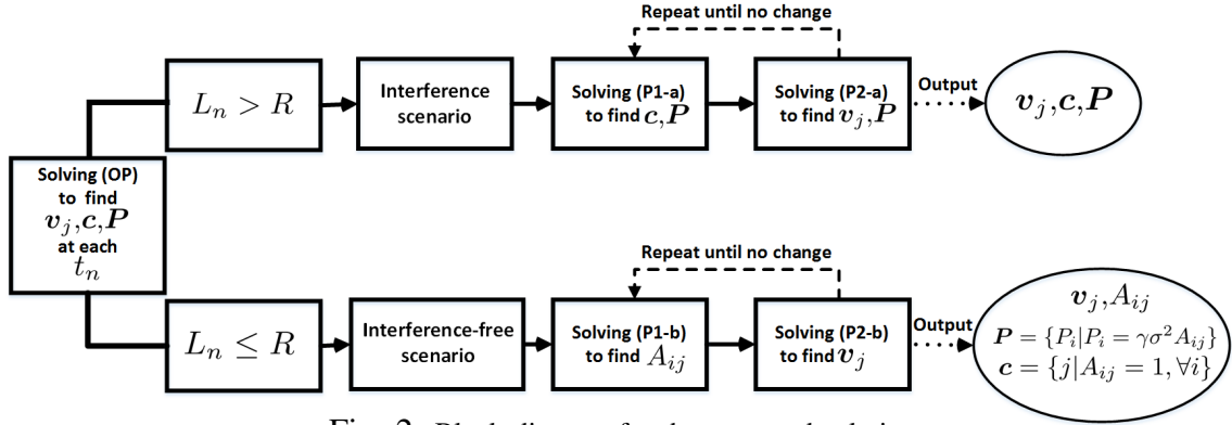
Fig. 2: Block diagram for the proposed solution.
