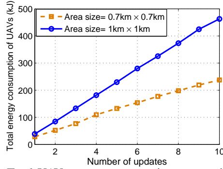
Fig. 12: Total UAV energy consumption vs. number of updates.
