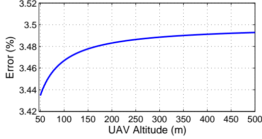
Fig. 3: Error in the objective function approximation.
