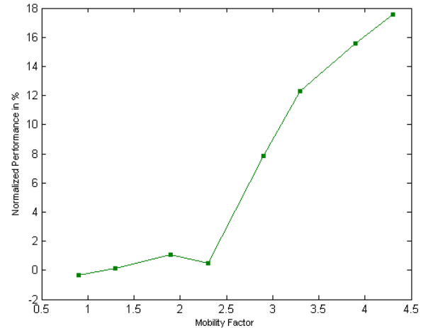
Figure 4 Performance of LEACH-ME over LEACH-M protocol.
