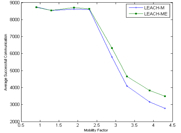
Figure 3 Average successful Communications of Leach-M and LEACH-ME for various mobility factors
