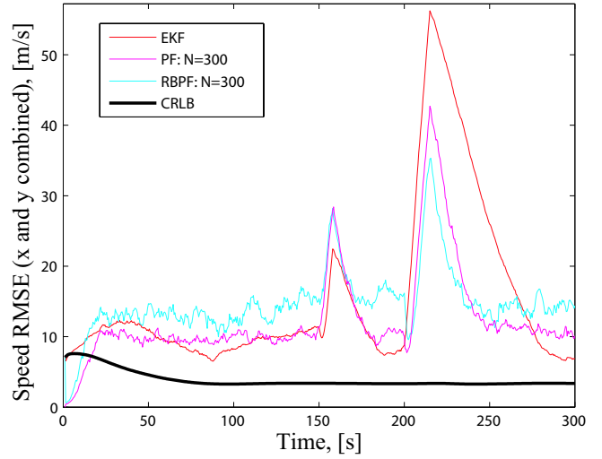
Fig. 5. RMSE of \dot{x} and \dot{y} speeds combined of the EKF, PF and RBPF (with N = 300 ) for N_{mc} = 100 runs.
