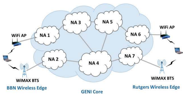
Fig. 16: GENI proof-of-concept demonstration topology
