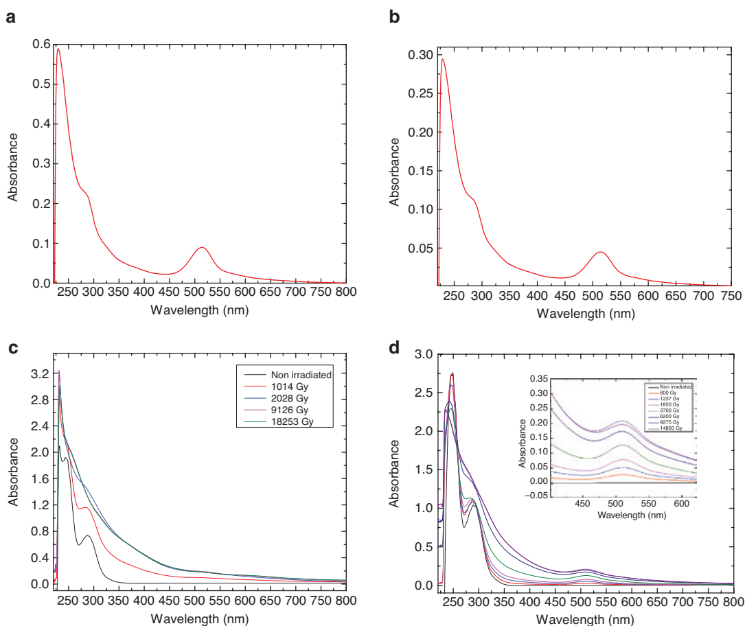
Figure 1: The figures a and b have been obtained after the chemical or electrochemical reductions Tc(VII)/Tc(IV) while in figures c and d, the evolution of the spectrum have been followed as a function of the dose.
