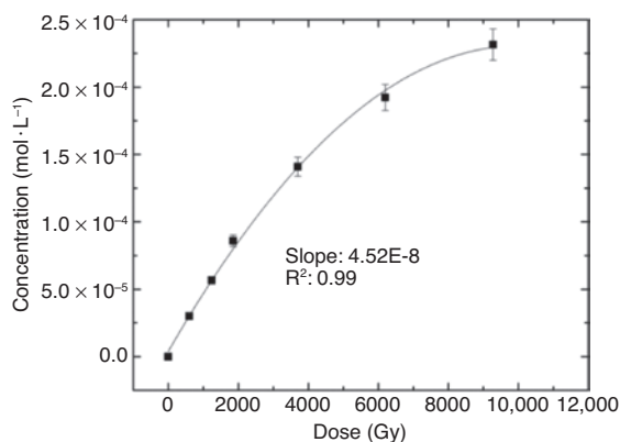
Figure 5: Concentration of obtained \text{Tc}_2(\mu - \text{O})_2 center product vs. dose obtained by \text{He}^{2+} radiolysis of [\text{Tc}(\text{VII})] = 5 \times 10^{-4} \text{ M} in carbonate solution [(\text{CO}_3^{2-}) = 5 \text{ M}, (\text{HCO}_3^-) = 0.5 \text{ M}, (\text{HCO}_2^-) = 0.7 \text{ M}] , dose rate = 1000 \text{ Gy} \cdot \text{min}^{-1} .
