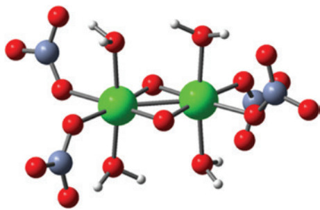
Figure 4: Calculated structure by DFT simulation of the technetium carbonate complex; technetium, oxygen, carbon and hydrogen atoms in green, red, gray and white colors; hydrogen bonds are showing in dotted mode with formula \text{Tc}_2(\mu - \text{O})_2(\text{CO}_3)_4(\text{OH}_2)_4 .
