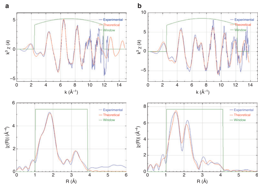
Figure 3: Figure a shows the EXAFS spectrum of the TcIV obtained by the chemical reduction while the figure b shows the EXAFS spectrum of TcIV obtained by the radiolytic one.
