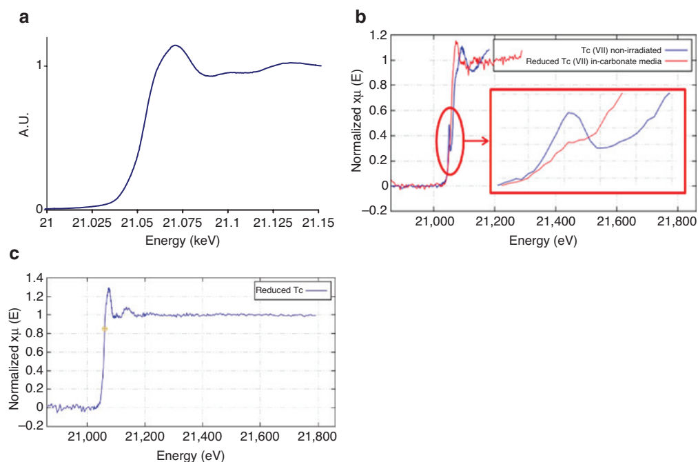
Figure 2: The figures a and c show the XANES spectrum of the TcIV while the figure b shows the XANES spectrum of TcVII before and after the irradiation experiment.
