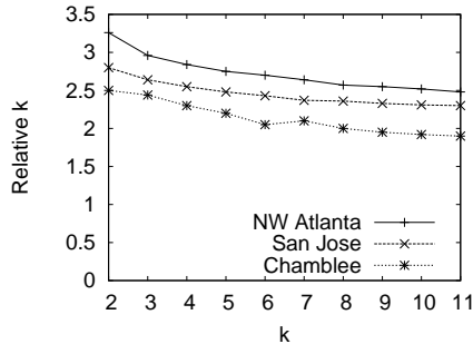
Fig. 10. Relative Anonymity
