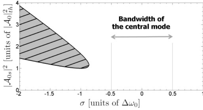
FIG. 5. Stability chart for the pumped mode and for the combs as a function of the laser detuning \sigma and the stationary pumped mode power |A_{0s}|^2 in the zero-dispersion case. The shaded area corresponds to unstable values of |A_{0s}|^2 [values destabilized by hysteresis, as explained in Fig. 4(c)] defined by Eq. (41). On the other hand, the hatched area corresponds to values of the pumped mode leading to stable comb generation, according to Eq. (52). Hence comb generation is only possible wherever the hatched area does not overlap the shaded area. Since both areas are perfectly overlapped, comb generation is impossible in the zero-dispersion case.
