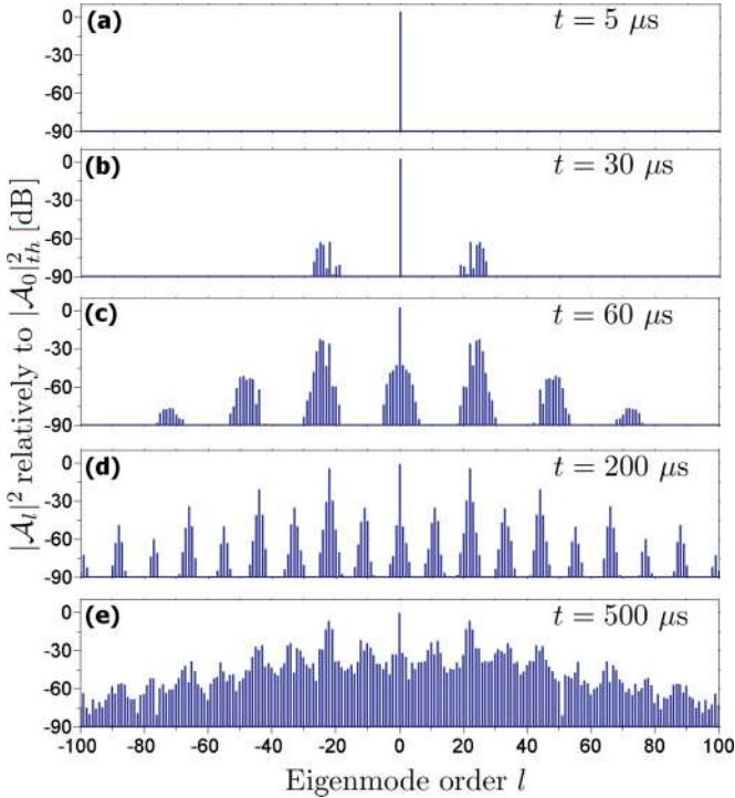
FIG. 11. (Color online) Transient dynamics of the comb when the cavity is pumped with |\mathcal{A}_{0s}|^2 = 1.8 |\mathcal{A}_{0th}|^2 . The parameters are \zeta = 2\pi \times 400 Hz and \sigma = 0 .
