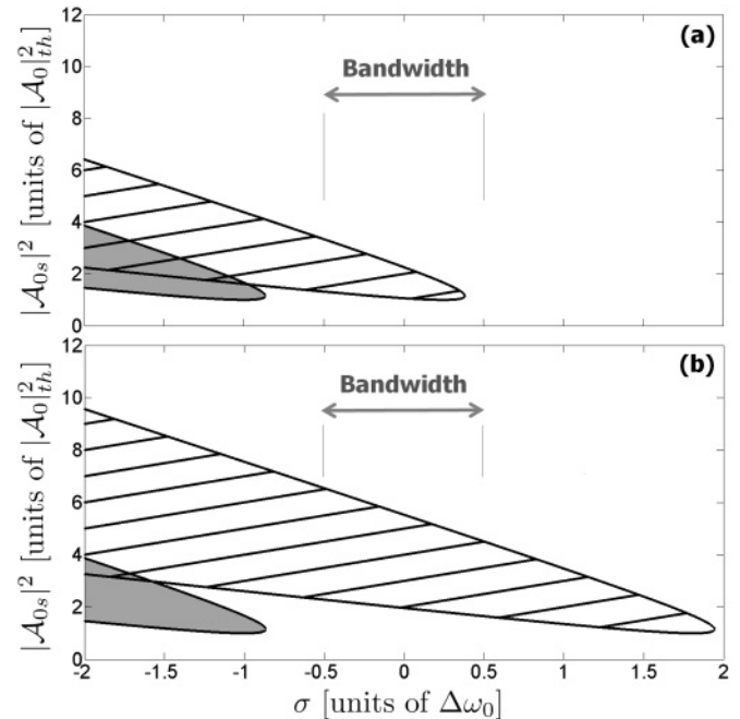
FIG. 7. Stability diagram of various pairs of side modes in the anomalous dispersion regime, with \zeta = 2\pi \times 400 Hz. Hatched and shaded areas have the same meaning as in Fig. 6, and this figure can be interpreted as a follow-up of Fig. 6(b) when the side mode order increases: (a) l = \pm 20 ; (b) l = \pm 30 .
