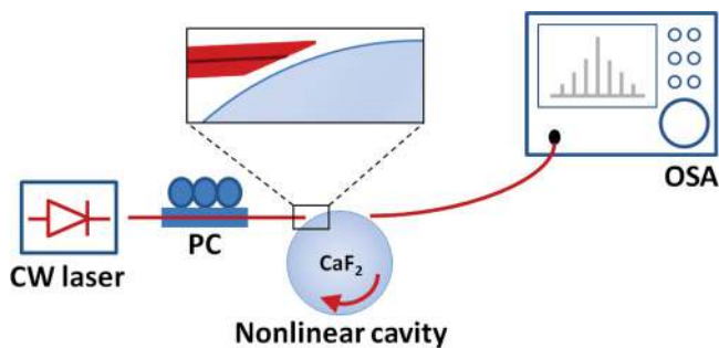
FIG. 1. (Color online) Optical-frequency comb generator with a calcium fluoride cavity and angle-polished fiber couplings. CW, continuous-wave; PC, polarization control; OSA, optical spectrum analyzer. The OSA displays the spectrum of the optical-frequency comb.
