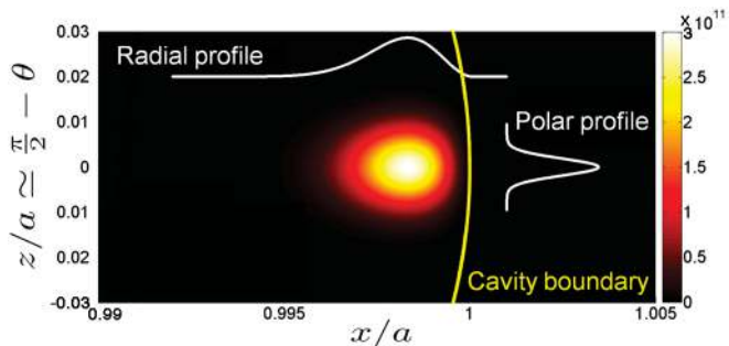
FIG. 2. (Color online) Cross section at \phi = 0 (half-plane y = 0 and x > 0 ) of the whispering gallery mode \|\Upsilon_{\ell, \text{TE}}(\mathbf{r})\|^2 in units of \text{m}^{-3} . The value of the polar eigennumber is \ell_0 = 14350 , corresponding to \lambda_0 = 1560.5 nm in vacuum. The spherical \text{CaF}_2 cavity has a radius a = 2.5 mm and a refractive index n_0 = 1.43 at \lambda_0 . Note that the axes are not orthonormal: the radial confinement is in fact 10 times stronger than the polar one.
