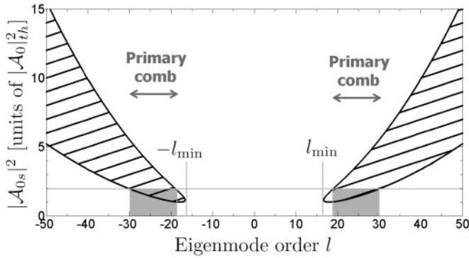
FIG. 8. An example of a stability diagram for comb generation as a function of eigenmode order l and power |A_{0s}|^2 in the central mode. The dispersion parameter is set to \zeta = 2\pi \times 400 Hz and the laser detuning to \sigma = 0 . The hatched area corresponds to stable comb generation, and the shaded areas are only there to emphasize the intervals hereinafter discussed. If the central mode is pumped twice above threshold, only the modes fulfilling 19 < |l| < 30 can be excited. No mode of order |l| < l_{\min} = 17 can be excited here through degenerate FWM.
