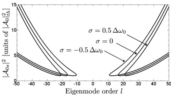
FIG. 9. Various stability diagrams for comb generation as a function of eigenmode order l and power |A_{0s}|^2 in the central mode, as the laser detuning \sigma is varied. The dispersion parameter is still set to \zeta = 2\pi \times 400 Hz, and the curve corresponding to \sigma = 0 is exactly the same as the one in Fig. 8. The hatchings have been omitted in this figure in order to improve its clarity.
