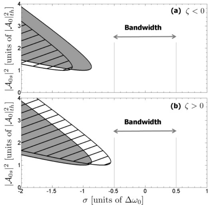
FIG. 6. Stability diagram for comb generation for the side modes l = \pm 10 . The shaded region still represents forbidden (unstable) values of the pumped mode, while the hatched areas correspond to those where a stable pump can effectively generate the comb. Stable comb generation effectively occurs in the hatched and nonshaded areas. Note that the shaded area does not change, but the hatched does. (a) Normal cavity dispersion \zeta = -2\pi \times 400 Hz. (b) Anomalous cavity dispersion \zeta = 2\pi \times 400 Hz.
