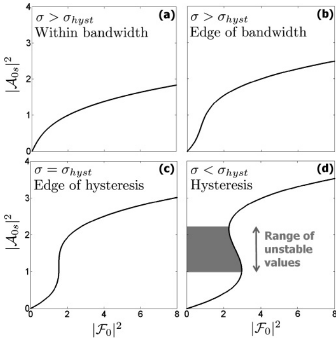
FIG. 4. Power |\mathcal{A}_{0s}|^2 in the pumped mode as a function of the injected power |\mathcal{F}_0|^2 , according to Eq. (38). Both variables are normalized in units of |\mathcal{A}_{0\text{th}}|^2 . The various figures correspond to different laser detuning frequencies \sigma . These amplitude variations are valid as long as no comb is generated in the system. (a) \sigma = 0 ; (b) \sigma = -0.5 \Delta\omega_0 ; (c) \sigma = -0.86 \Delta\omega_0 ; (d) \sigma = -1.2 \Delta\omega_0 .
