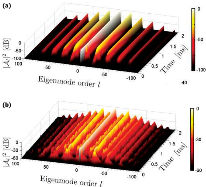
FIG. 12. (Color online) Spectrotemporal behavior of the full comb with \zeta = 2\pi \times 400 Hz and \sigma = 0 . (a) |\mathcal{A}_{0s}|^2 = 1.2 |\mathcal{A}_{0th}|^2 , the spectral components converge toward constant values; (b) |\mathcal{A}_{0s}|^2 = 1.8 |\mathcal{A}_{0th}|^2 , the spectrum is chaotic in the time domain. Note that snapshots at t = 2 ms would correspond to Figs. 10(b) and 10(c), respectively.
