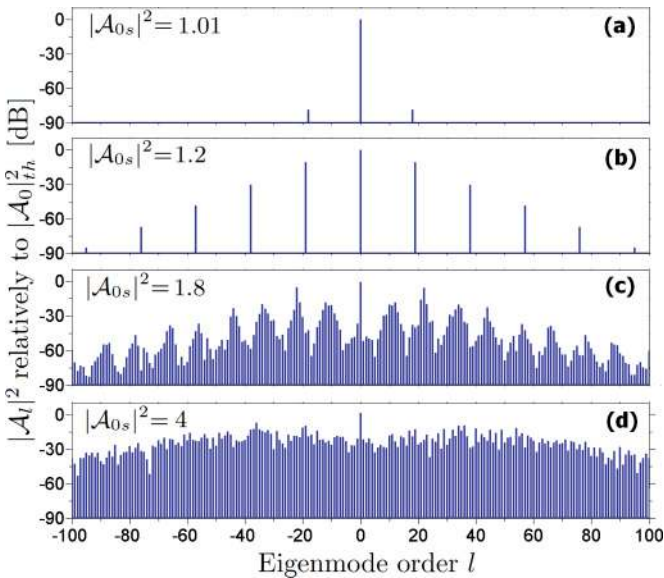
FIG. 10. (Color online) Evolution of the full comb as the pump power in the central mode is increased. The displayed combs correspond to spectrum snapshots at t = 2 ms. The parameters are \zeta = 2\pi \times 400 Hz and \sigma = 0 . The |\mathcal{A}_{0s}|^2 is expressed in units of the threshold power |\mathcal{A}_0|_{\text{th}}^2 .
