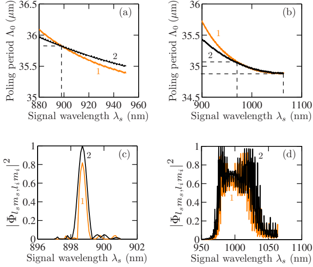
FIG. 5. (Color online) A laser source with wavelength \lambda_p = 532 nm and in mode l_p m_p = -11 is used to pump a poled silica fiber with \Delta=0.01 . [(a) and (b)] Poling period versus the signal wavelength \lambda_s , with core radii a=2.613 and a=2.52 \mu\text{m} , respectively. The orange (black) curve represents condition 1 (2), namely, that the signal (idler) mode number l_s m_s (l_i m_i) is 01 and the idler (signal) mode number l_i m_i (l_s m_s) is 11. Dashed lines show the intersection point or region. [(c) and (d)] These panels display modal/spectral entanglement regimes. Normalized output spectra |\Phi_{01,11}(\omega_s)|^2 and |\Phi_{11,01}(\omega_s)|^2 for the structures displayed in (a) and (b), respectively, with L=20 cm. The poling period of the nonlinear coefficient is uniform in (c) with \Lambda_0=35.813 \mu\text{m} , and is linearly chirped in (d) with \Lambda_0=34.9 \mu\text{m} and \Lambda_L=35.05 \mu\text{m} .
