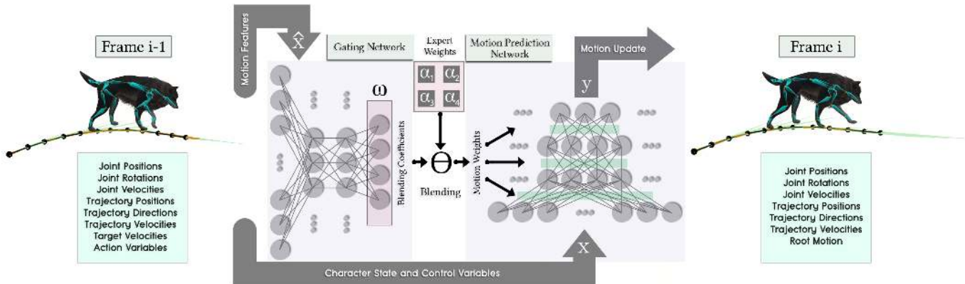
Fig. 3. The architecture of our neural network composed of the gating network and the motion prediction network. The gating network takes as input the current end effector velocities of the feet, the desired velocity and the action vector. The motion prediction network takes as input the posture and trajectory control variables from the previous frame, and predicts the updated posture and trajectory for the current frame.
