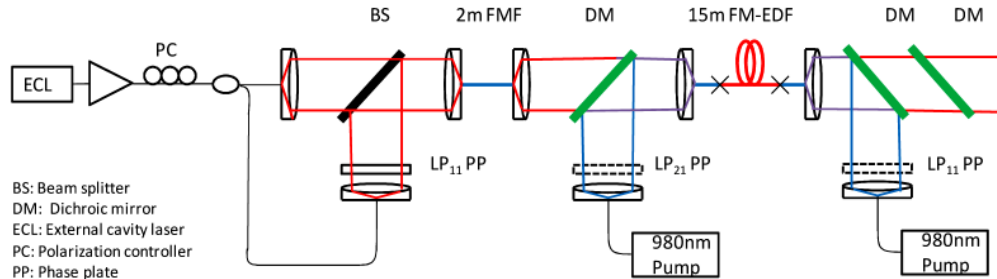
Fig. 2. Experiment setup.
