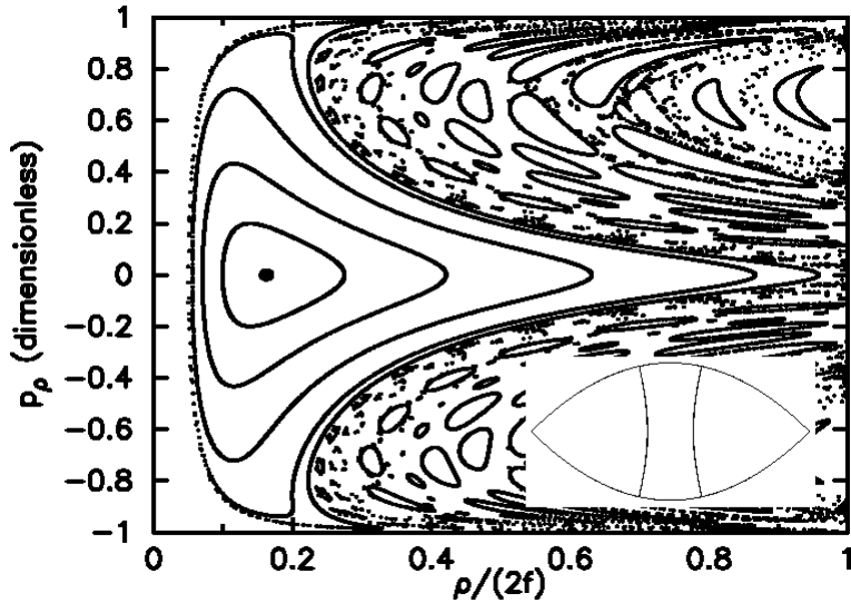
Figure 14: Surface of section at L_z = 0.1 f with \varepsilon = -0.02 f . The cavity develops a multitude of stable periodic orbits surrounded by elliptical islands. The most prominent island of stability is centered on the the line p_\rho = 0 where a small circle indicates the location of the corresponding periodic orbit around which other trajectories can oscillate. Shown in the inset is the central stable periodic orbit. The next innermost closed line in the SOS belongs to the trajectory shown in Fig. 13 (c).
