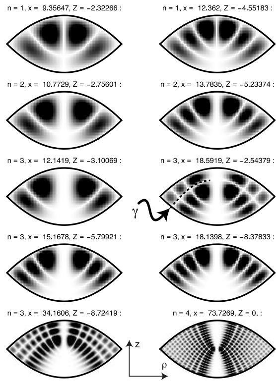
Figure 9: Mode intensities as in Fig. 8, but without performing the symmetrization prescribed by the focal plane boundary condition. The WKB quantum numbers \mu (and \nu ) can be read off by counting the number of wavefunction nodes parallel (and perpendicular) to the reference line \gamma . Modes in the first three rows correspond to the symmetrized versions of Fig. 8. In order to illustrate the approach to the short-wavelength limit, additional modes are shown for which the formation of caustics is apparent in the high-intensity ridges (black) bordering the classically forbidden regions (white).
