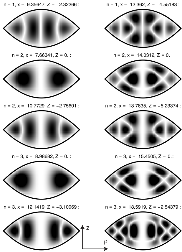
Figure 8: The modes shown here do not follow the simple law of Eq. (56) but were obtained numerically. With increasing centrifugal barrier, labeled by n , the forbidden region around the z -axis grows outward.
