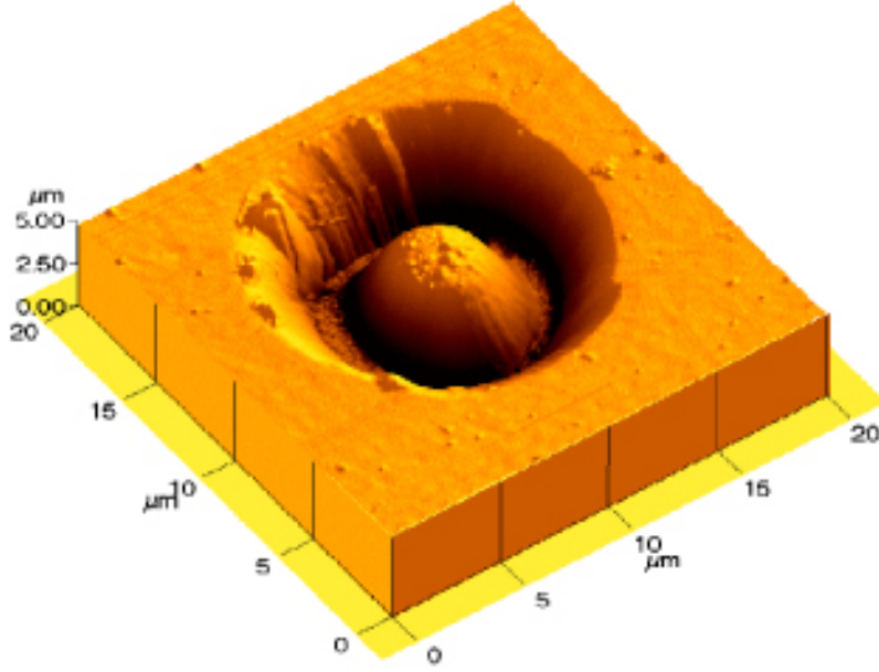
Figure 1: Atomic Force Microscope image of a “hill” of diameter 7.2 \mu\text{m} and parabolic cross-section of height 1.8 \mu\text{m} , etched on a GaAs substrate by a Focused Ion Beam apparatus. When covered with gold it constitutes a concave parabolic mirror with its focal point inside the GaAs substrate.
