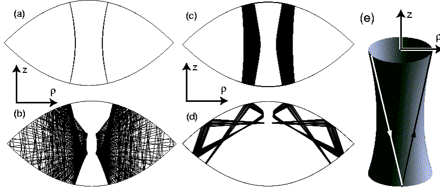
Figure 13: Trajectories in the non-confocal cavity. (a) shows the unstable periodic orbit arising at \varepsilon = 0.02f , L_z = 0.1f , cf. Fig. 12. For the same parameter, a chaotic trajectory is seen in (b). Oscillatory motion around stable periodic orbits occurs in (c) and (d), where \varepsilon = -0.02f and L_z = 0.1f as in the SOS of Fig. 14. The patterns of type (a) and (c) derive from the periodic motion of Fig. 10 (a) as a result of the shape perturbation. In real three-dimensional cartesian space, (e) shows the straight-line ray motion (arrows) giving rise to the curved “envelope” surface whose cross section we see in (a).
