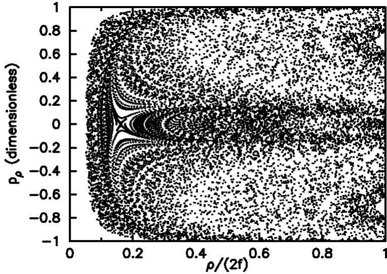
Figure 12: Surface of section at L_z = 0.1 f of a non-confocal double-paraboloid, with foci pulled apart by \varepsilon = 0.02 f . This destabilizes the cavity, leading to chaotic ray dynamics which generates an irregular cloud of points filling almost the whole region that is accessible for this L_z . A special point is encountered on the line p_\rho = 0 where the irregularity gives way to a confluence of hyperbolic traces whose vertices are centered on a single, unstable periodic orbit. The spatial pattern of this new periodic orbit is shown in Fig. 13 (a).
