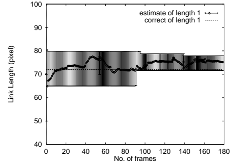
Fig.11. Estimates of the 1st link length r_1
