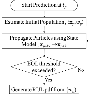
Figure 4. Prediction flowchart.
