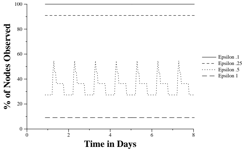
Fig. 7 Figure showing the number of sensors observed over time for varying epsilons for value queries with a 95% confidence on the garden data.
