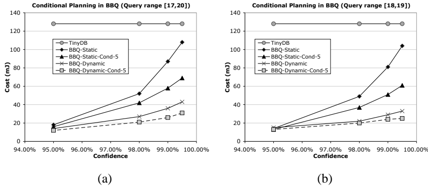
Fig. 16 Conditional planning experiments on the garden data: We plot the energy costs of various query evaluation techniques for two range queries, \langle 17, 20 \rangle , and \langle 18, 19 \rangle .
