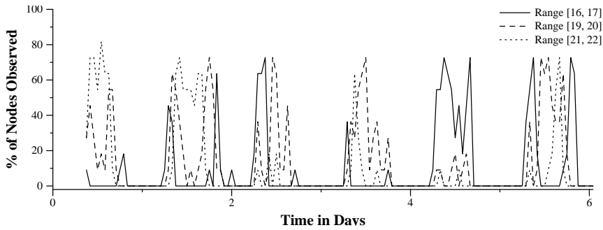
Fig. 13 Graph showing BBQ’s performance on three different range queries, for the garden data set with confidence set to 95%.
