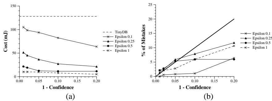
Fig. 12 Energy per query (a) and percentage of errors (b) versus confidence interval size and epsilon, for average queries on the garden data.
