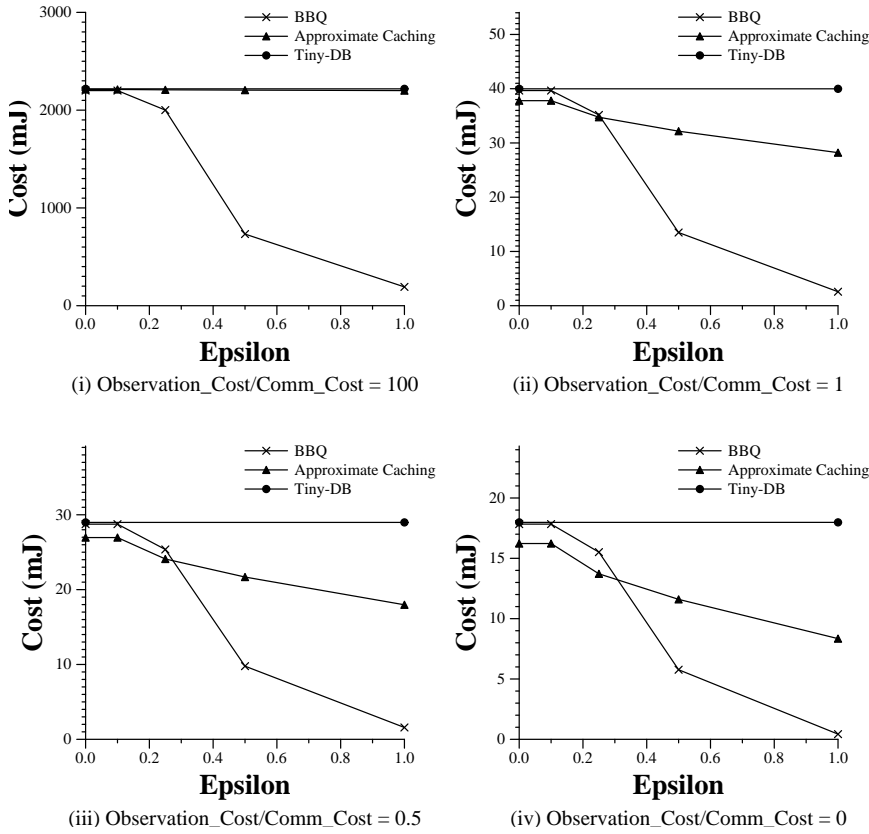
Fig. 8 Comparing the effectiveness of the algorithms for varying ratios of communication and observation costs. As we can see, over a wide range of ratios, the performance of BBQ is significantly better than either of the other two techniques. Note that the y-axes are plotted on different scales across the graphs.
