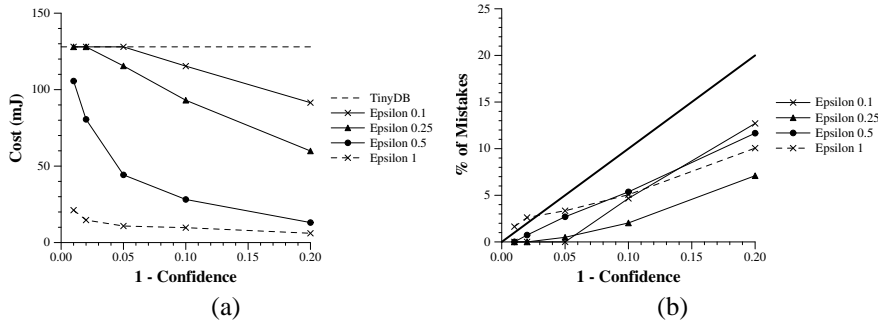
Fig. 9 Energy per query (a) and percentage of errors (b) versus confidence interval size and epsilon, for value queries on the garden data. The 45^\circ line in (b) represents the target number of mistakes for the given confidence level, points below this line have made less mistakes than the confidence bounds allow them to make.
