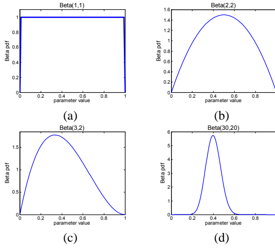
Fig. 19 Bayesian approach for learning the parameter of a coin: (a) prior distribution, Beta(1,1); posterior distributions over the coin parameter after observing: (b) 1 head, 1 tail; (c) 2 heads, 1 tail; (d) 29 heads, 19 tails.
