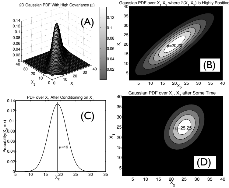
Fig. 3 Example of Gaussians: (a) 3D plot of a 2D Gaussian with high covariance; (b) the same Gaussian viewed as a contour plot; (c) the resulting Gaussian over X_2 after a particular value of X_1 has been observed; finally, (d) shows how, as uncertainty about X_1 increases from the time we last observed it, we again have a 2D Gaussian with a lower variance and shifted mean.
