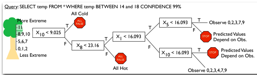
Fig. 17 Example of a conditional plan generated by BBQ on the garden data.
