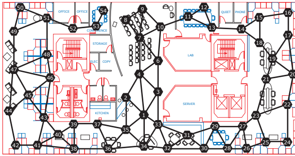
Fig. 18 Structure of graphical model learned for the temperature variables for a deployment in the Intel Berkeley Lab [45].
