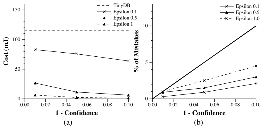
Fig. 14 Energy per query (a) and percentage of errors (b) versus confidence interval size and epsilon for the Lab Data.
