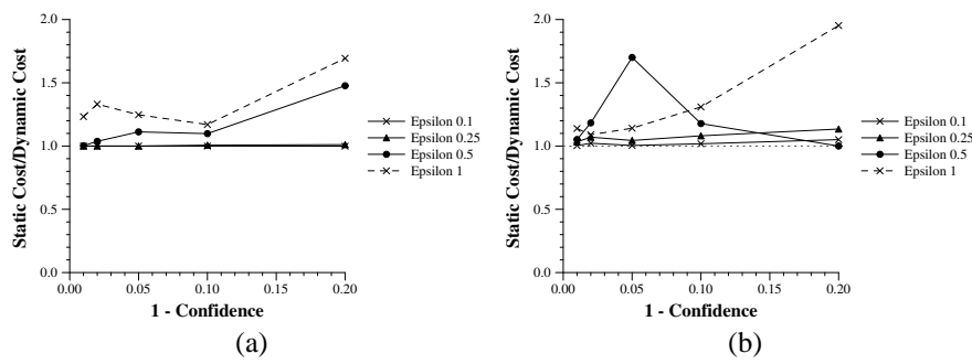
Fig. 11 Ratio of costs of dynamic vs static for value and average queries on the garden data.
