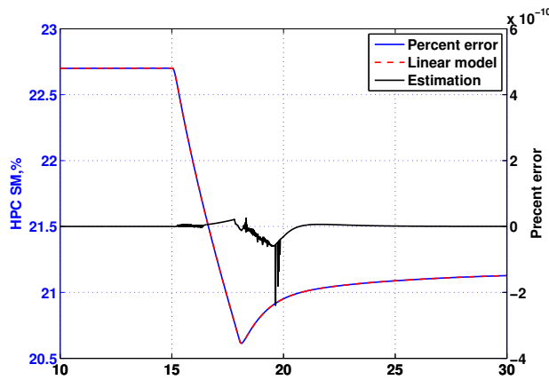
Figure 6. Verification of the optimal tuner estimation to be able to track an open loop stall margin transient from the linear model at 50% deterioration.
