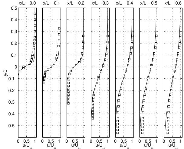
Figure 3: Velocity profiles for the cavity shear layer. Hot wire measurements ( \square ) and tanh profiles with same vorticity thickness and deflection ( \text{—} ).
