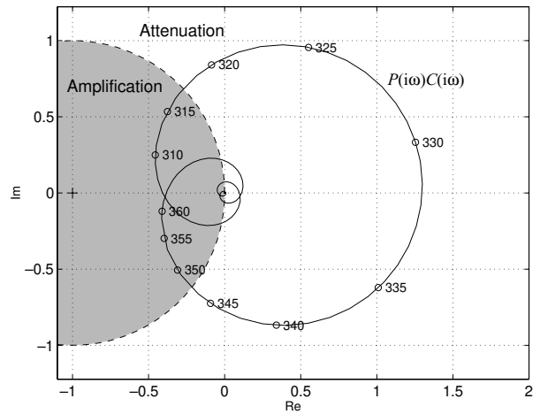
Figure 13: Nyquist plot for the feedback system, along with corresponding frequencies (in Hz). Points outside the dashed circle correspond to a performance benefit ( |S(i\omega)| < 1 ), and points inside the circle correspond to a penalty ( |S(i\omega)| > 1 ).
