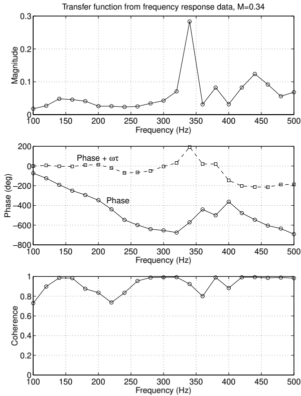
Figure 10: Transfer function from input voltage to pressure measured by Kulite 8, measured from frequency response experiment at M = 0.34 . Also shown is the phase with a time delay of \tau = 8 ms removed.
