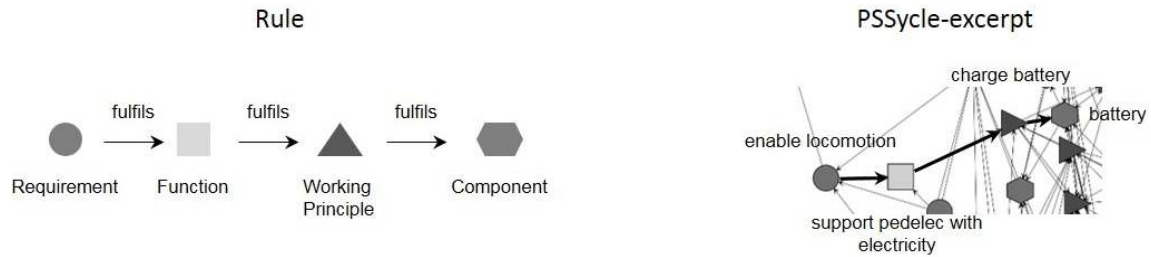
Figure 5. Example: rule-based modeling
